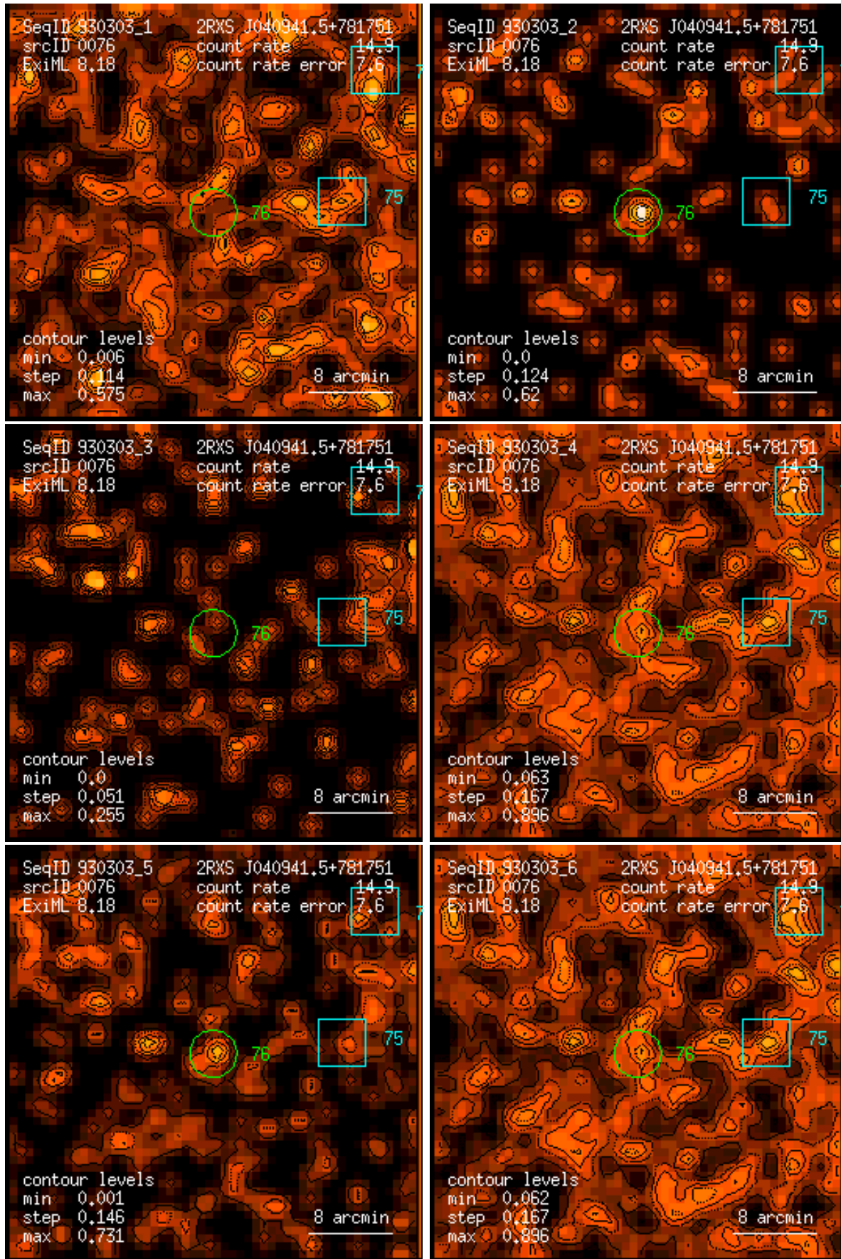
Figure 76: RASS 930303: detection 0076: band rate images, Gaussian filter: (1) PSPC channels 11 – 41, (2) 52 – 90, (3) 91 – 201, (4) 11 – 235, (5) 52 – 201, (6) 11 – 201. Broad band rates in counts/ks. Band rate contour levels in counts/ks/arcmin 2 .
