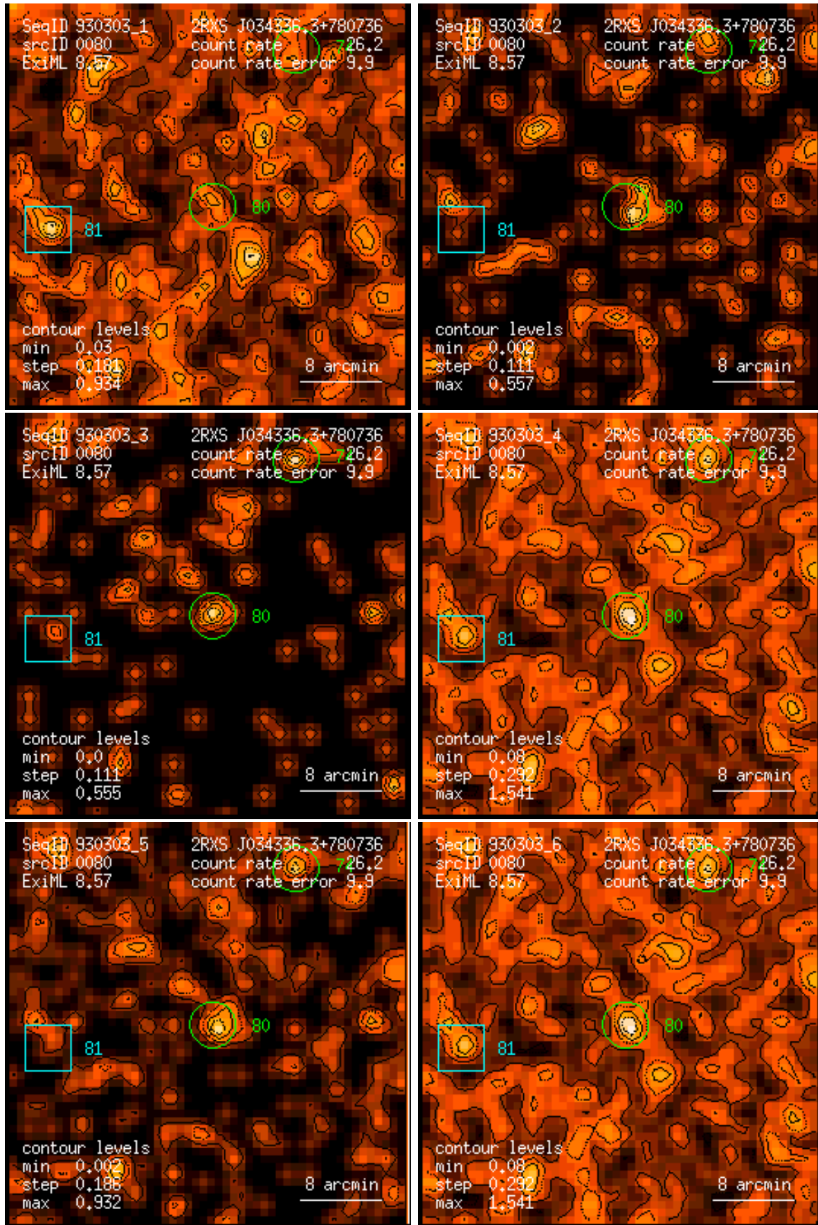
Figure 80: RASS 930303: detection 0080: band rate images, Gaussian filter: (1) PSPC channels 11 – 41, (2) 52 – 90, (3) 91 – 201, (4) 11 – 235, (5) 52 – 201, (6) 11 – 201. Broad band rates in counts/ks. Band rate contour levels in counts/ks/arcmin 2 .
