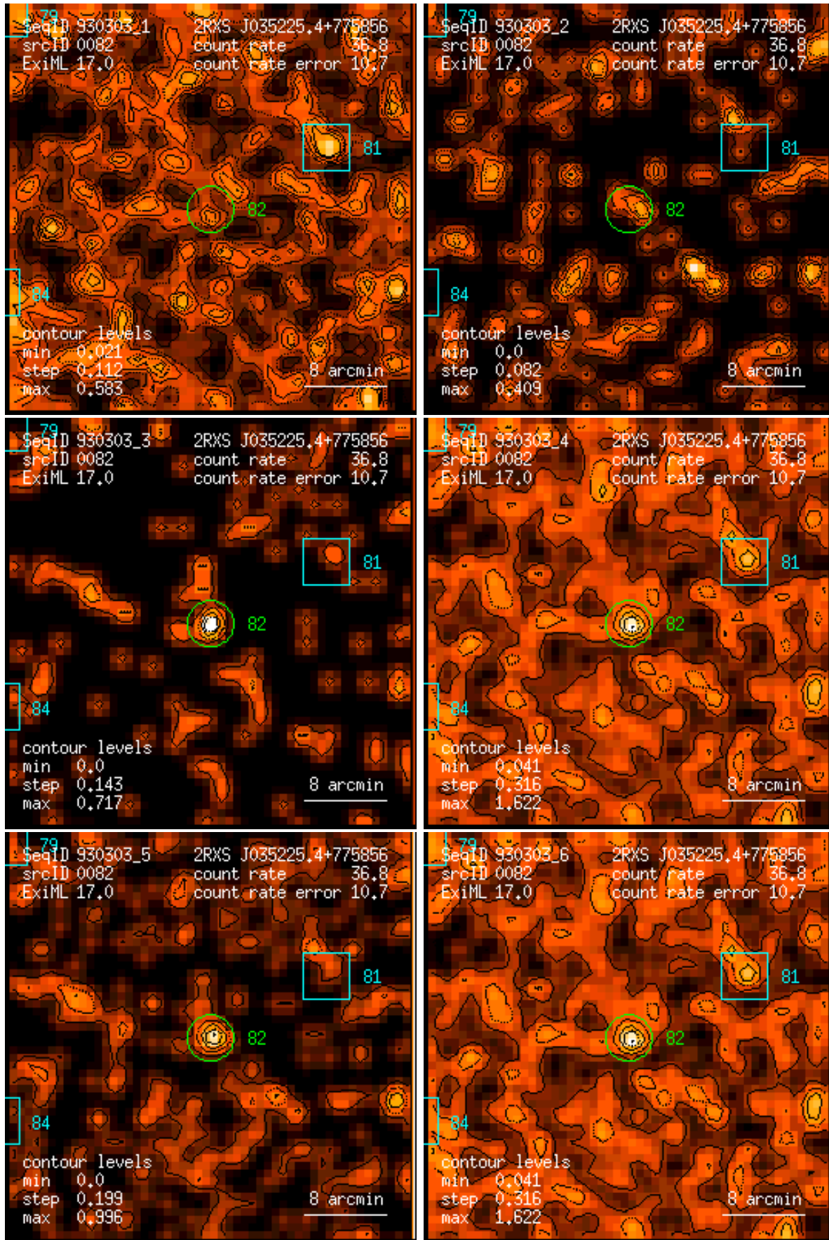
Figure 82: RASS 930303: detection 0082: band rate images, Gaussian filter: (1) PSPC channels 11 – 41, (2) 52 – 90, (3) 91 – 201, (4) 11 – 235, (5) 52 – 201, (6) 11 – 201. Broad band rates in counts/ks. Band rate contour levels in counts/ks/arcmin 2 .
