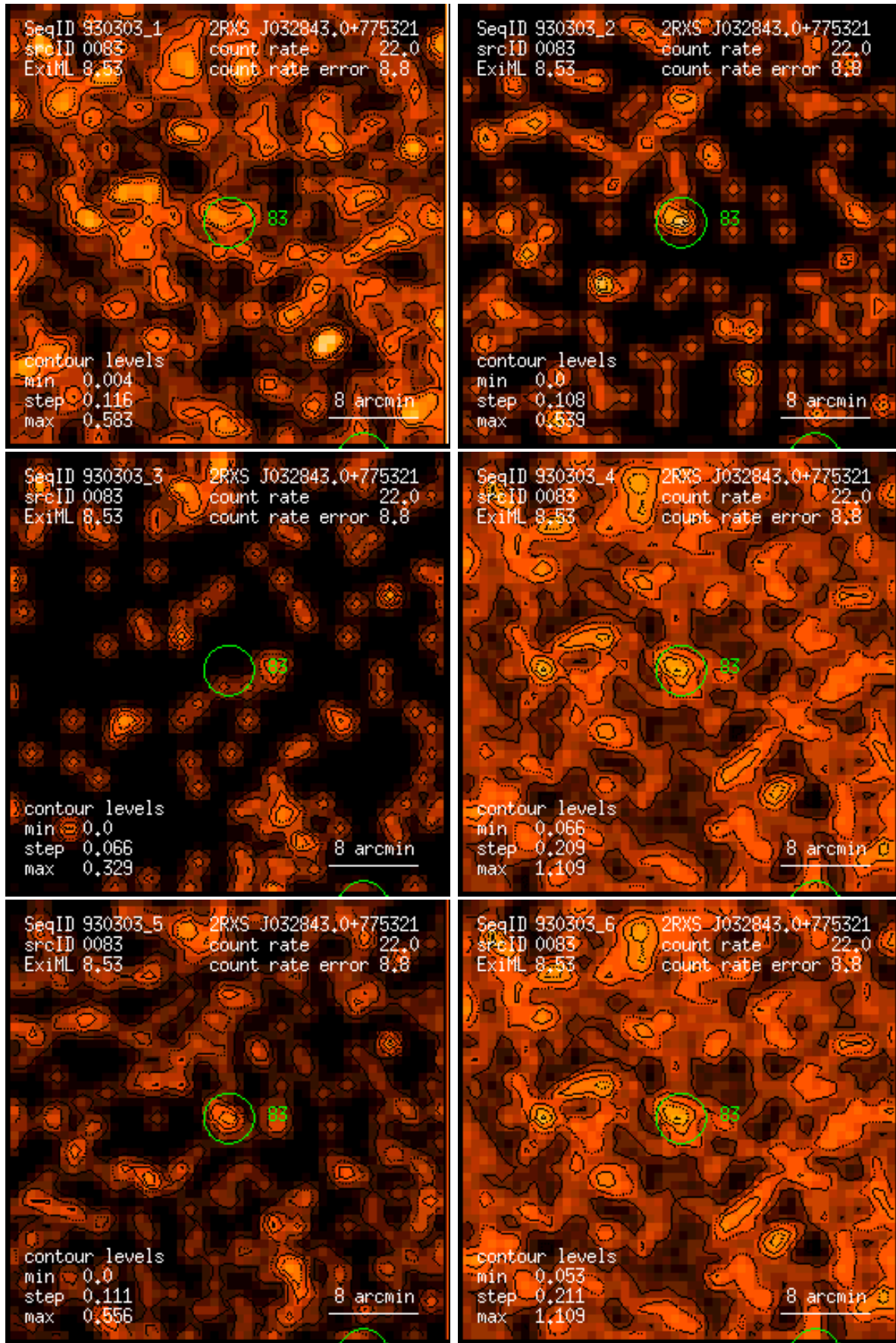
Figure 83: RASS 930303: detection 0083: band rate images, Gaussian filter: (1) PSPC channels 11 – 41, (2) 52 – 90, (3) 91 – 201, (4) 11 – 235, (5) 52 – 201, (6) 11 – 201. Broad band rates in counts/ks. Band rate contour levels in counts/ks/arcmin 2 .
