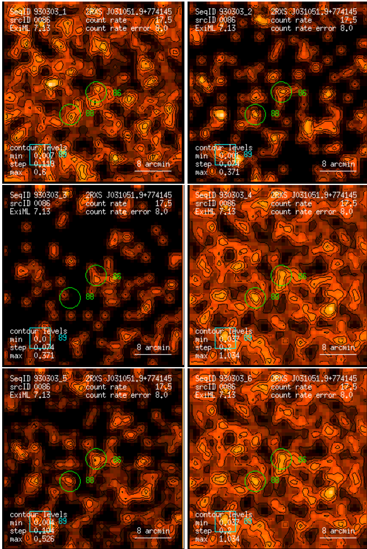
Figure 86: RASS 930303: detection 0086: band rate images, Gaussian filter: (1) PSPC channels 11 – 41, (2) 52 – 90, (3) 91 – 201, (4) 11 – 235, (5) 52 – 201, (6) 11 – 201. Broad band rates in counts/ks. Band rate contour levels in counts/ks/arcmin 2 .
