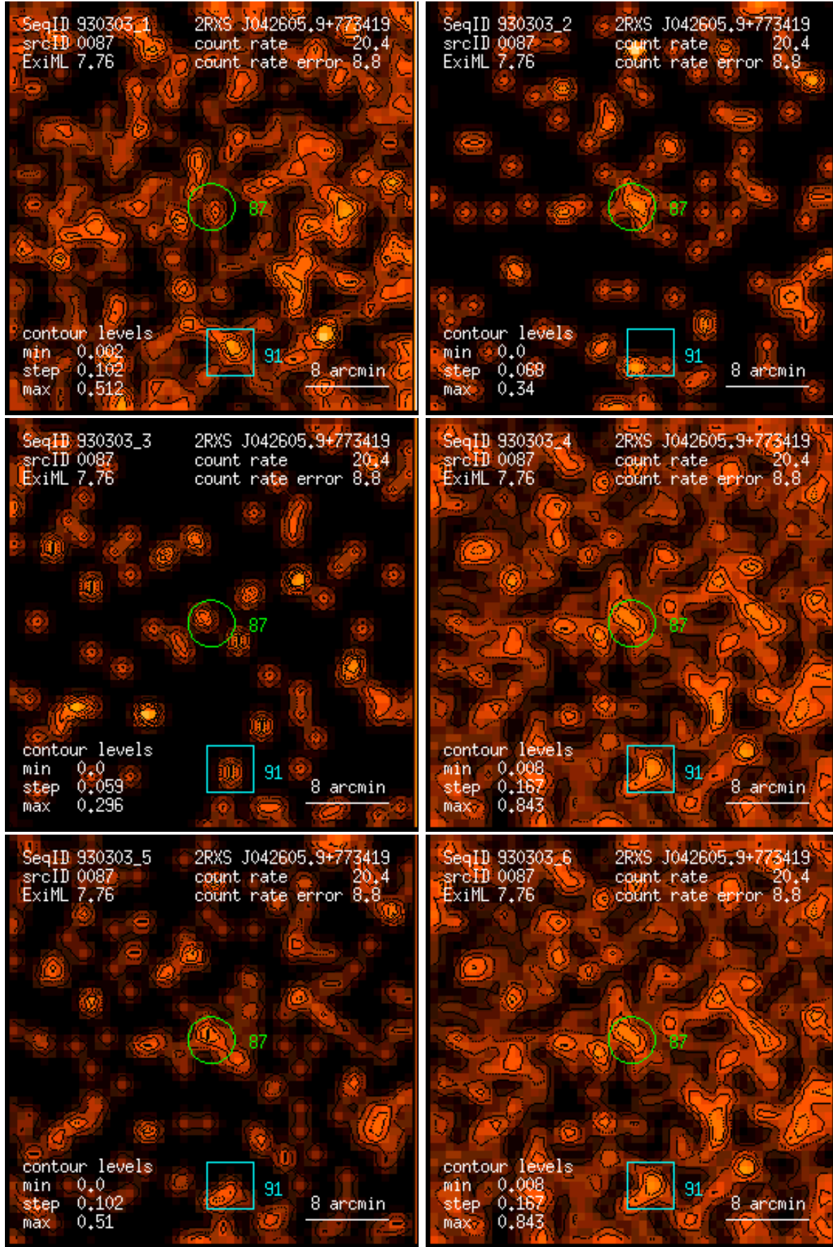
Figure 87: RASS 930303: detection 0087: band rate images, Gaussian filter: (1) PSPC channels 11 – 41, (2) 52 – 90, (3) 91 – 201, (4) 11 – 235, (5) 52 – 201, (6) 11 – 201. Broad band rates in counts/ks. Band rate contour levels in counts/ks/arcmin 2 .
