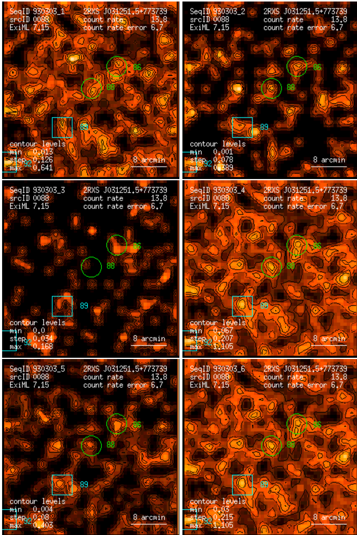
Figure 88: RASS 930303: detection 0088: band rate images, Gaussian filter: (1) PSPC channels 11 – 41, (2) 52 – 90, (3) 91 – 201, (4) 11 – 235, (5) 52 – 201, (6) 11 – 201. Broad band rates in counts/ks. Band rate contour levels in counts/ks/arcmin 2 .
