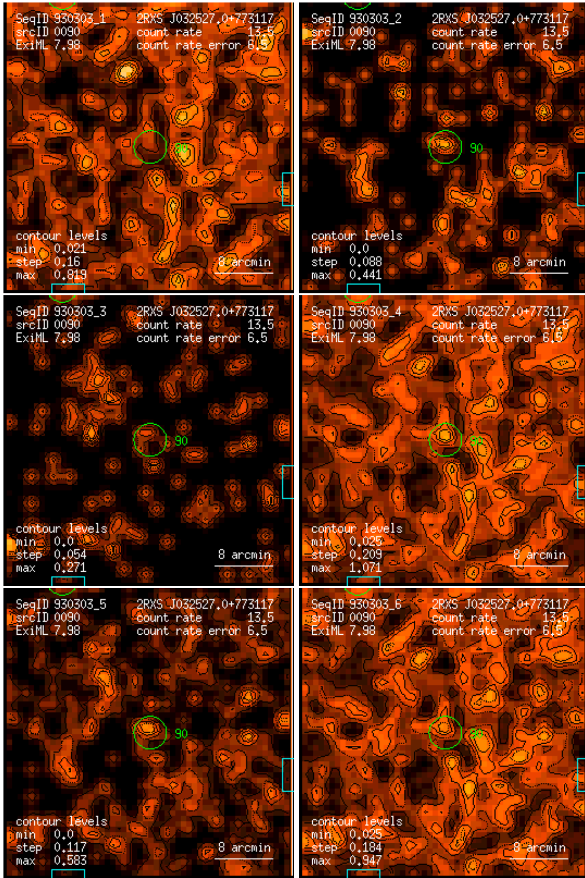
Figure 90: RASS 930303: detection 0090: band rate images, Gaussian filter: (1) PSPC channels 11 – 41, (2) 52 – 90, (3) 91 – 201, (4) 11 – 235, (5) 52 – 201, (6) 11 – 201. Broad band rates in counts/ks. Band rate contour levels in counts/ks/arcmin 2 .
