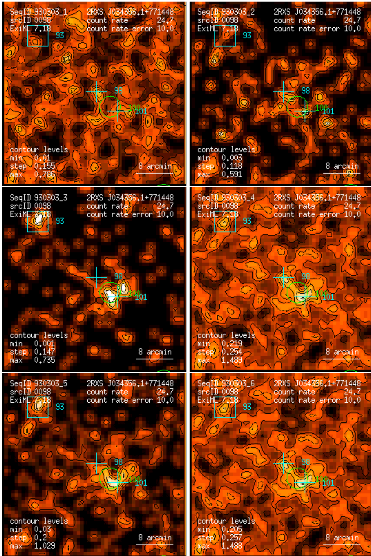
Figure 98: RASS 930303: detection 0098: band rate images, Gaussian filter: (1) PSPC channels 11 – 41, (2) 52 – 90, (3) 91 – 201, (4) 11 – 235, (5) 52 – 201, (6) 11 – 201. Broad band rates in counts/ks. Band rate contour levels in counts/ks/arcmin 2 .
