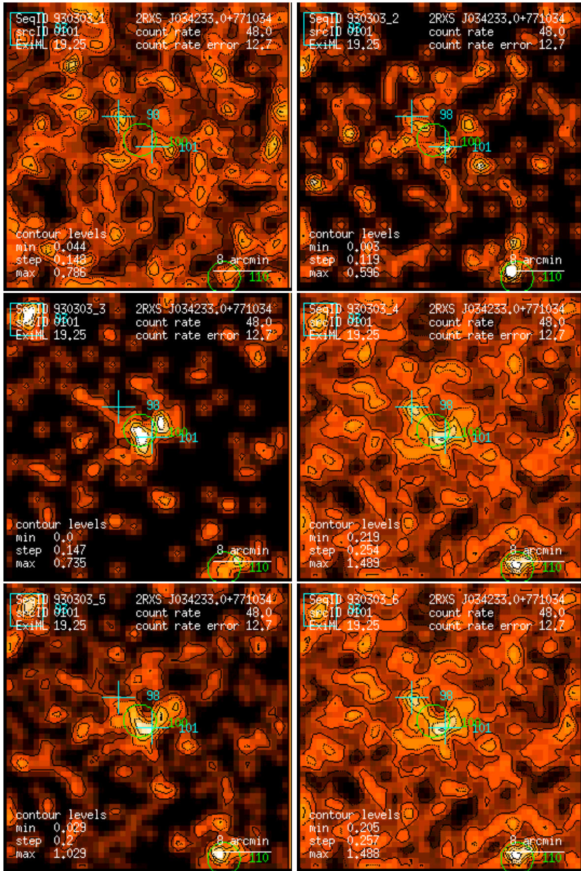
Figure 101: RASS 930303: detection 0101: band rate images, Gaussian filter: (1) PSPC channels 11 – 41, (2) 52 – 90, (3) 91 – 201, (4) 11 – 235, (5) 52 – 201, (6) 11 – 201. Broad band rates in counts/ks. Band rate contour levels in counts/ks/arcmin 2 .
