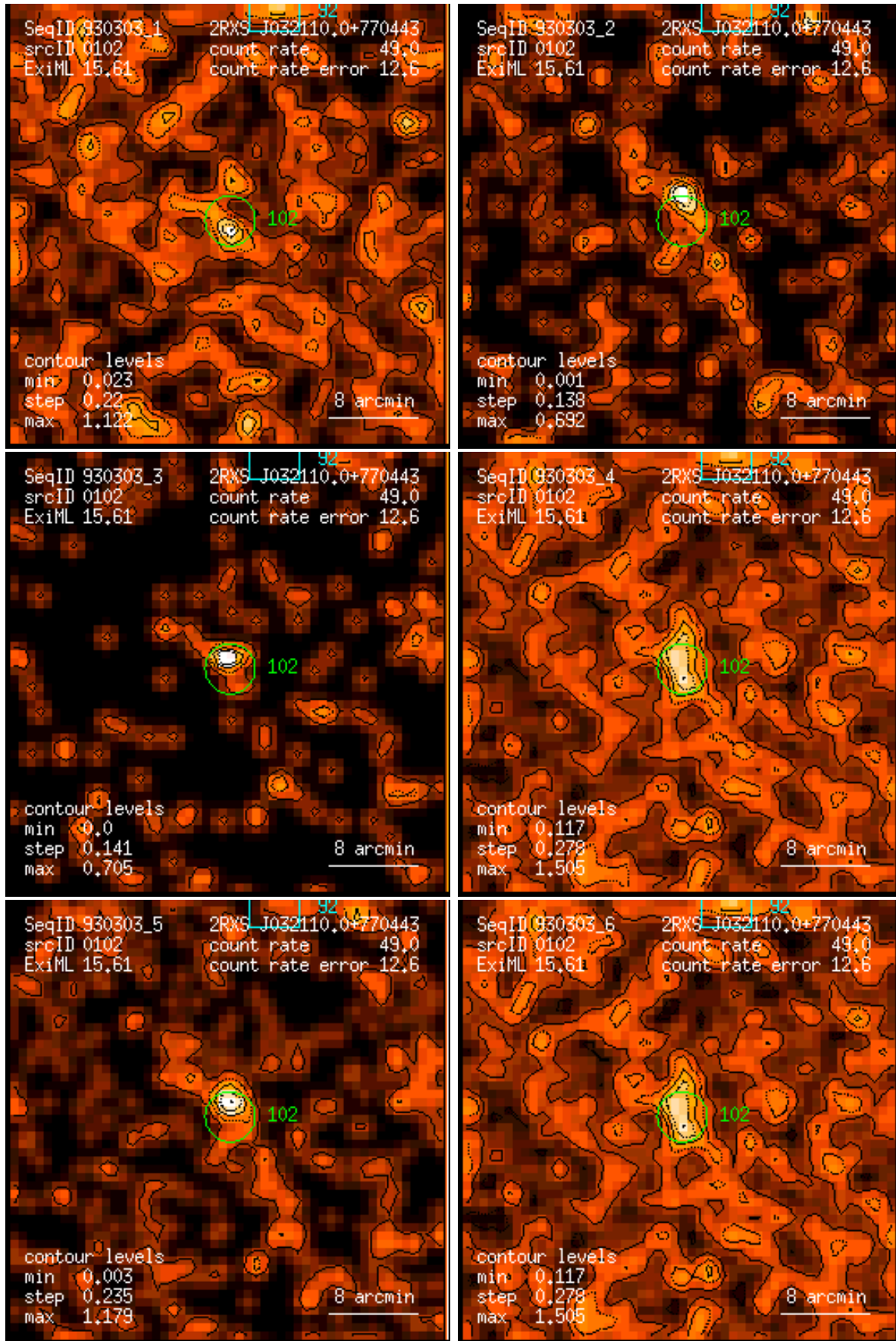
Figure 102: RASS 930303: detection 0102: band rate images, Gaussian filter: (1) PSPC channels 11 – 41, (2) 52 – 90, (3) 91 – 201, (4) 11 – 235, (5) 52 – 201, (6) 11 – 201. Broad band rates in counts/ks. Band rate contour levels in counts/ks/arcmin 2 .
