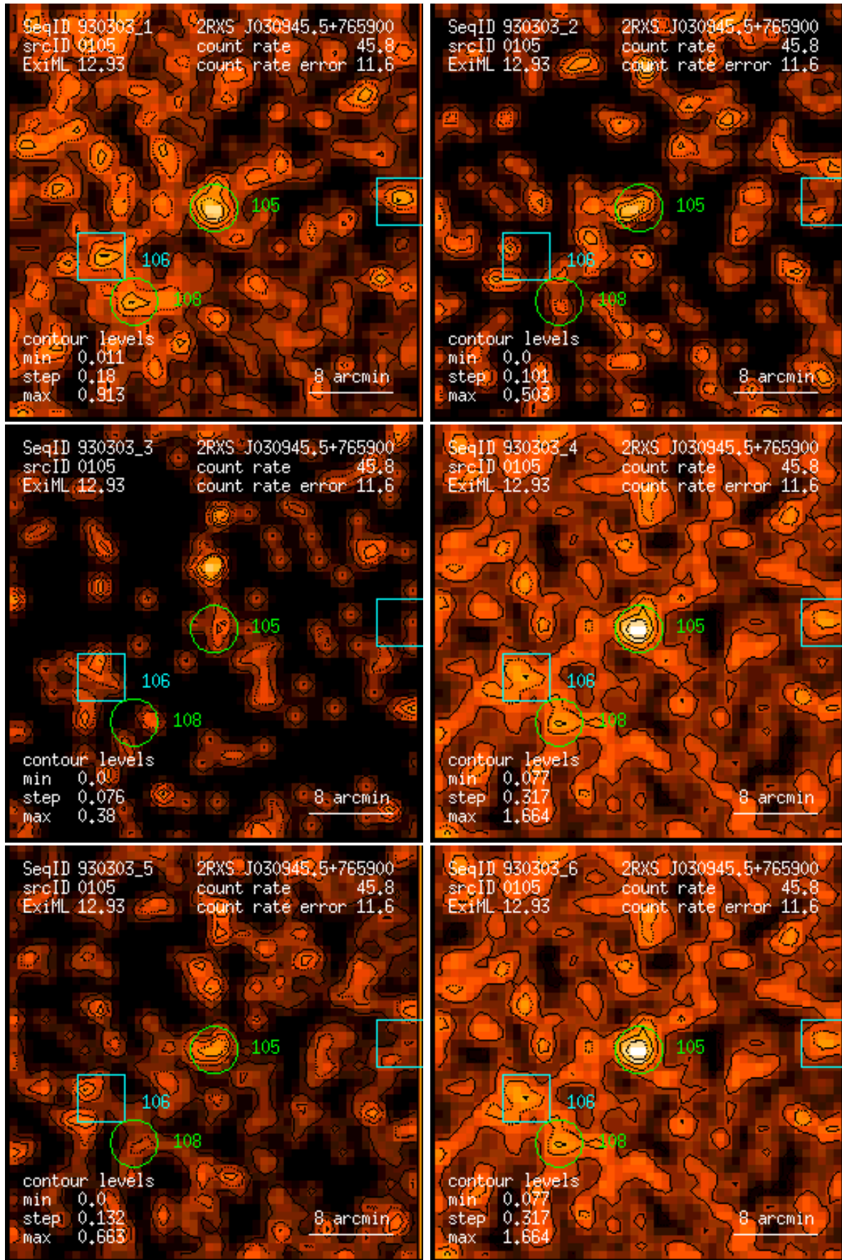
Figure 105: RASS 930303: detection 0105: band rate images, Gaussian filter: (1) PSPC channels 11 – 41, (2) 52 – 90, (3) 91 – 201, (4) 11 – 235, (5) 52 – 201, (6) 11 – 201. Broad band rates in counts/ks. Band rate contour levels in counts/ks/arcmin 2 .
