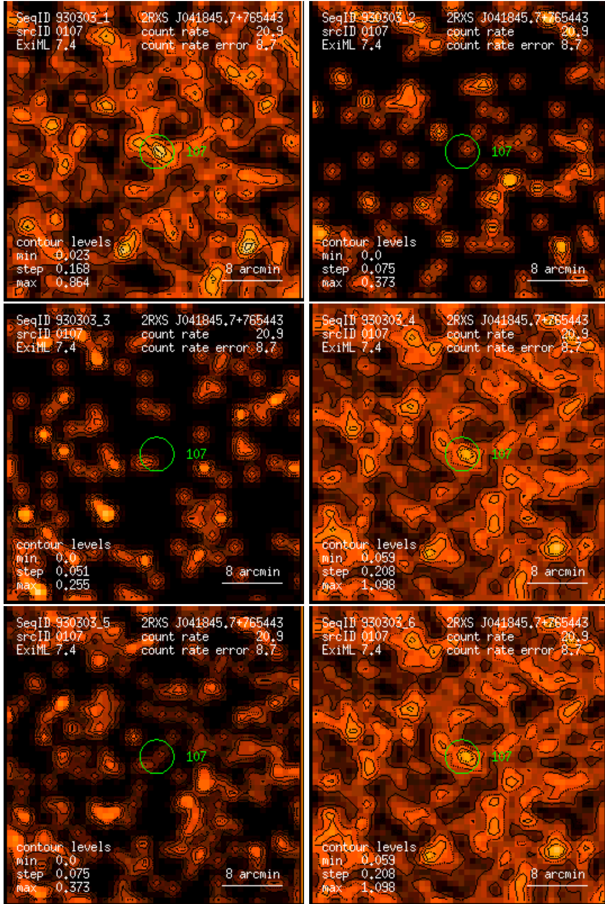
Figure 107: RASS 930303: detection 0107: band rate images, Gaussian filter: (1) PSPC channels 11 – 41, (2) 52 – 90, (3) 91 – 201, (4) 11 – 235, (5) 52 – 201, (6) 11 – 201. Broad band rates in counts/ks. Band rate contour levels in counts/ks/arcmin 2 .
