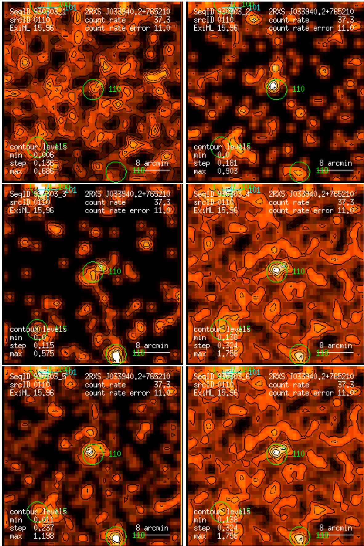
Figure 110: RASS 930303: detection 0110: band rate images, Gaussian filter: (1) PSPC channels 11 – 41, (2) 52 – 90, (3) 91 – 201, (4) 11 – 235, (5) 52 – 201, (6) 11 – 201. Broad band rates in counts/ks. Band rate contour levels in counts/ks/arcmin 2 .
