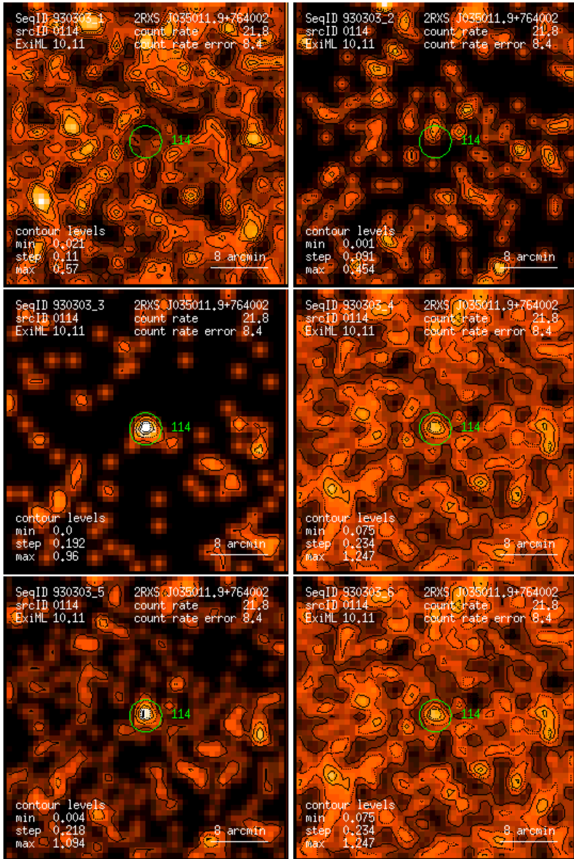
Figure 114: RASS 930303: detection 0114: band rate images, Gaussian filter: (1) PSPC channels 11 – 41, (2) 52 – 90, (3) 91 – 201, (4) 11 – 235, (5) 52 – 201, (6) 11 – 201. Broad band rates in counts/ks. Band rate contour levels in counts/ks/arcmin 2 .
