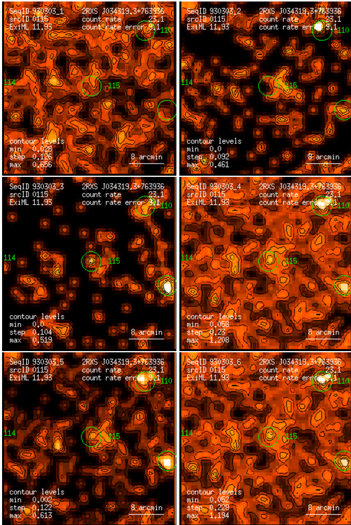
Figure 115: RASS 930303: detection 0115: band rate images, Gaussian filter: (1) PSPC channels 11 – 41, (2) 52 – 90, (3) 91 – 201, (4) 11 – 235, (5) 52 – 201, (6) 11 – 201. Broad band rates in counts/ks. Band rate contour levels in counts/ks/arcmin 2 .
