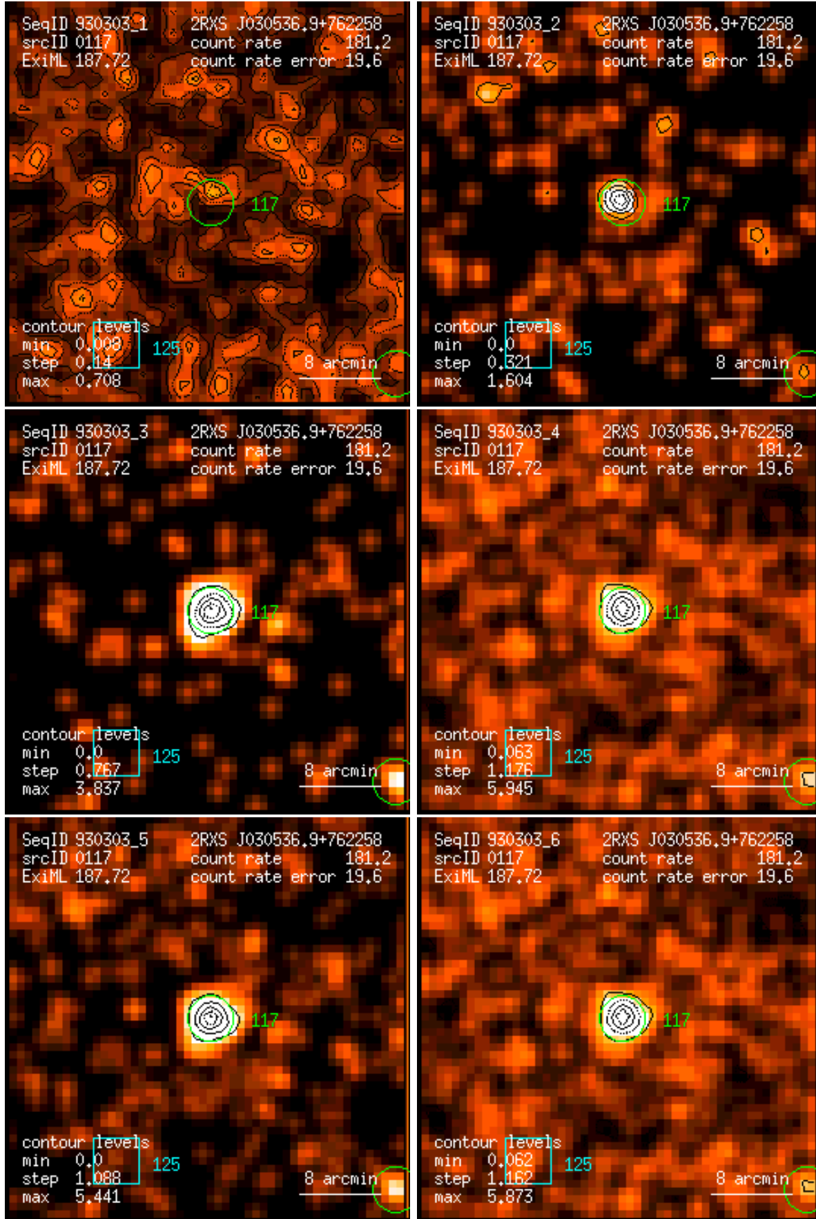
Figure 117: RASS 930303: detection 0117: band rate images, Gaussian filter: (1) PSPC channels 11 – 41, (2) 52 – 90, (3) 91 – 201, (4) 11 – 235, (5) 52 – 201, (6) 11 – 201. Broad band rates in counts/ks. Band rate contour levels in counts/ks/arcmin 2 .
