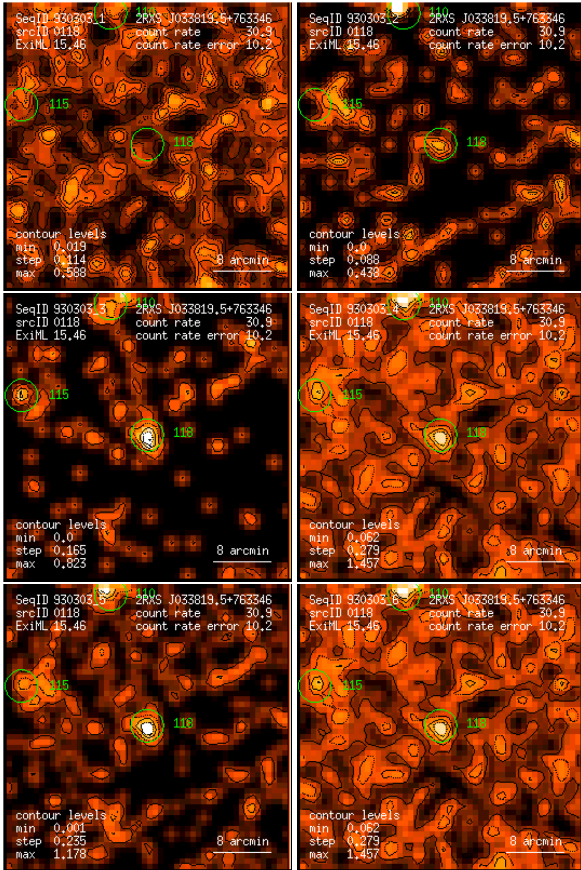
Figure 118: RASS 930303: detection 0118: band rate images, Gaussian filter: (1) PSPC channels 11 – 41, (2) 52 – 90, (3) 91 – 201, (4) 11 – 235, (5) 52 – 201, (6) 11 – 201. Broad band rates in counts/ks. Band rate contour levels in counts/ks/arcmin 2 .
