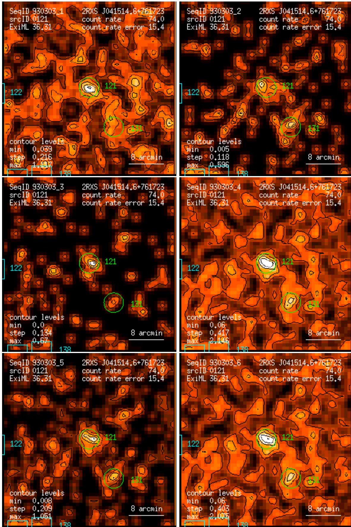
Figure 121: RASS 930303: detection 0121: band rate images, Gaussian filter: (1) PSPC channels 11 – 41, (2) 52 – 90, (3) 91 – 201, (4) 11 – 235, (5) 52 – 201, (6) 11 – 201. Broad band rates in counts/ks. Band rate contour levels in counts/ks/arcmin 2 .
