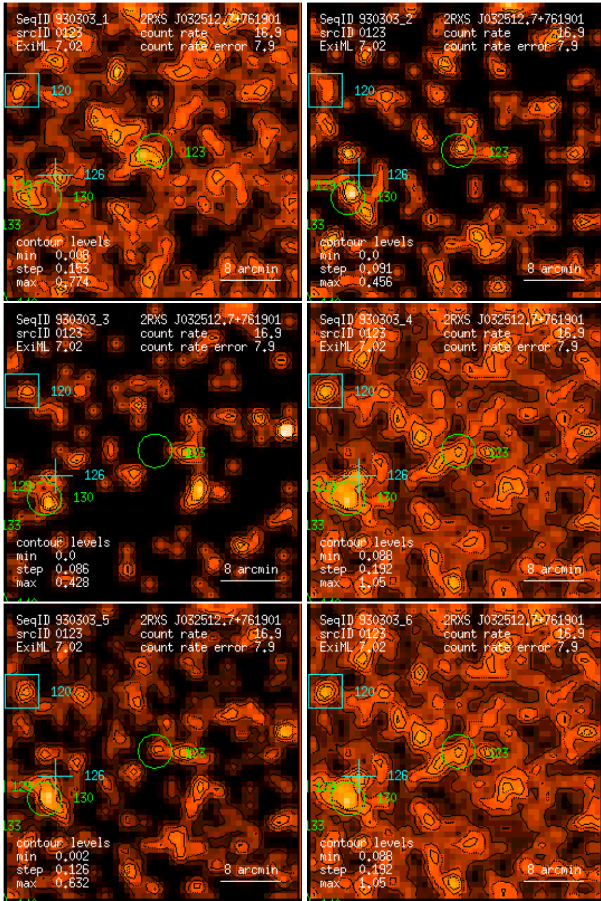
Figure 123: RASS 930303: detection 0123: band rate images, Gaussian filter: (1) PSPC channels 11 – 41, (2) 52 – 90, (3) 91 – 201, (4) 11 – 235, (5) 52 – 201, (6) 11 – 201. Broad band rates in counts/ks. Band rate contour levels in counts/ks/arcmin 2 .
