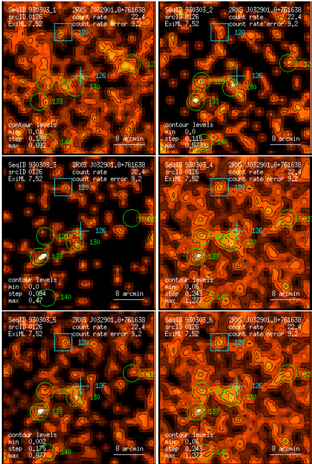
Figure 126: RASS 930303: detection 0126: band rate images, Gaussian filter: (1) PSPC channels 11 – 41, (2) 52 – 90, (3) 91 – 201, (4) 11 – 235, (5) 52 – 201, (6) 11 – 201. Broad band rates in counts/ks. Band rate contour levels in counts/ks/arcmin 2 .
