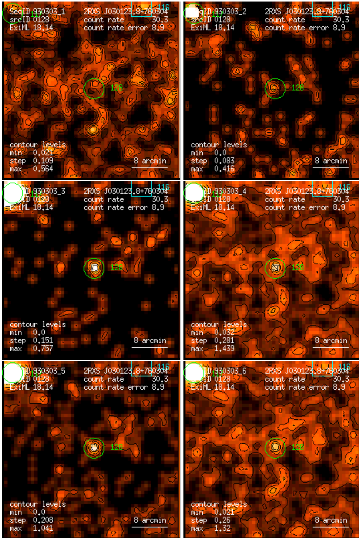
Figure 128: RASS 930303: detection 0128: band rate images, Gaussian filter: (1) PSPC channels 11 – 41, (2) 52 – 90, (3) 91 – 201, (4) 11 – 235, (5) 52 – 201, (6) 11 – 201. Broad band rates in counts/ks. Band rate contour levels in counts/ks/arcmin 2 .
