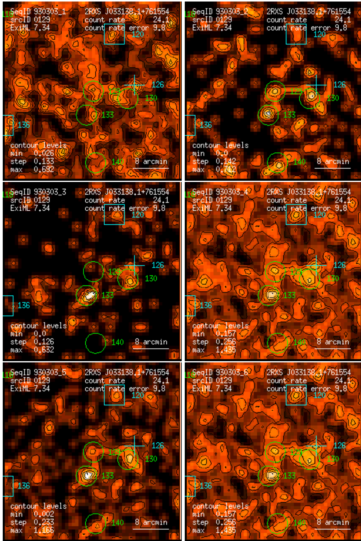
Figure 129: RASS 930303: detection 0129: band rate images, Gaussian filter: (1) PSPC channels 11 – 41, (2) 52 – 90, (3) 91 – 201, (4) 11 – 235, (5) 52 – 201, (6) 11 – 201. Broad band rates in counts/ks. Band rate contour levels in counts/ks/arcmin 2 .
