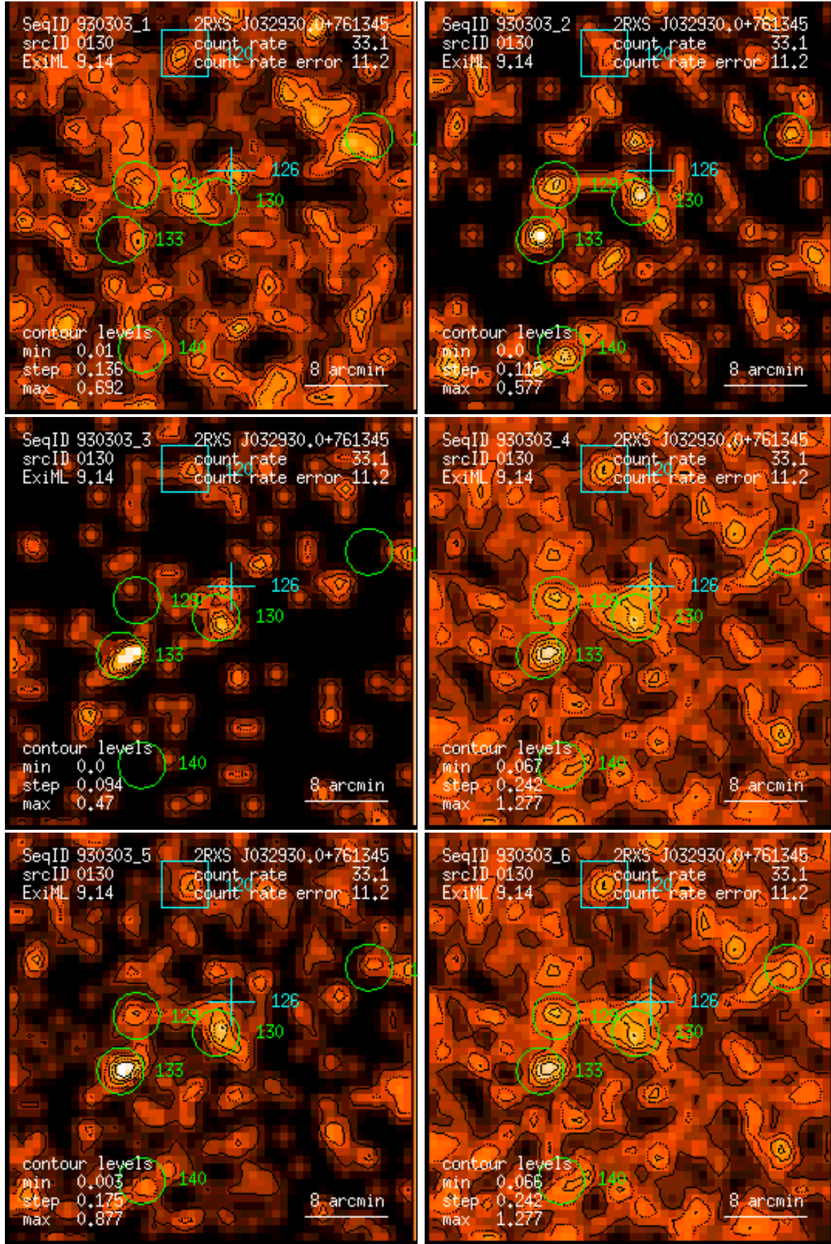
Figure 130: RASS 930303: detection 0130: band rate images, Gaussian filter: (1) PSPC channels 11 – 41, (2) 52 – 90, (3) 91 – 201, (4) 11 – 235, (5) 52 – 201, (6) 11 – 201. Broad band rates in counts/ks. Band rate contour levels in counts/ks/arcmin 2 .
