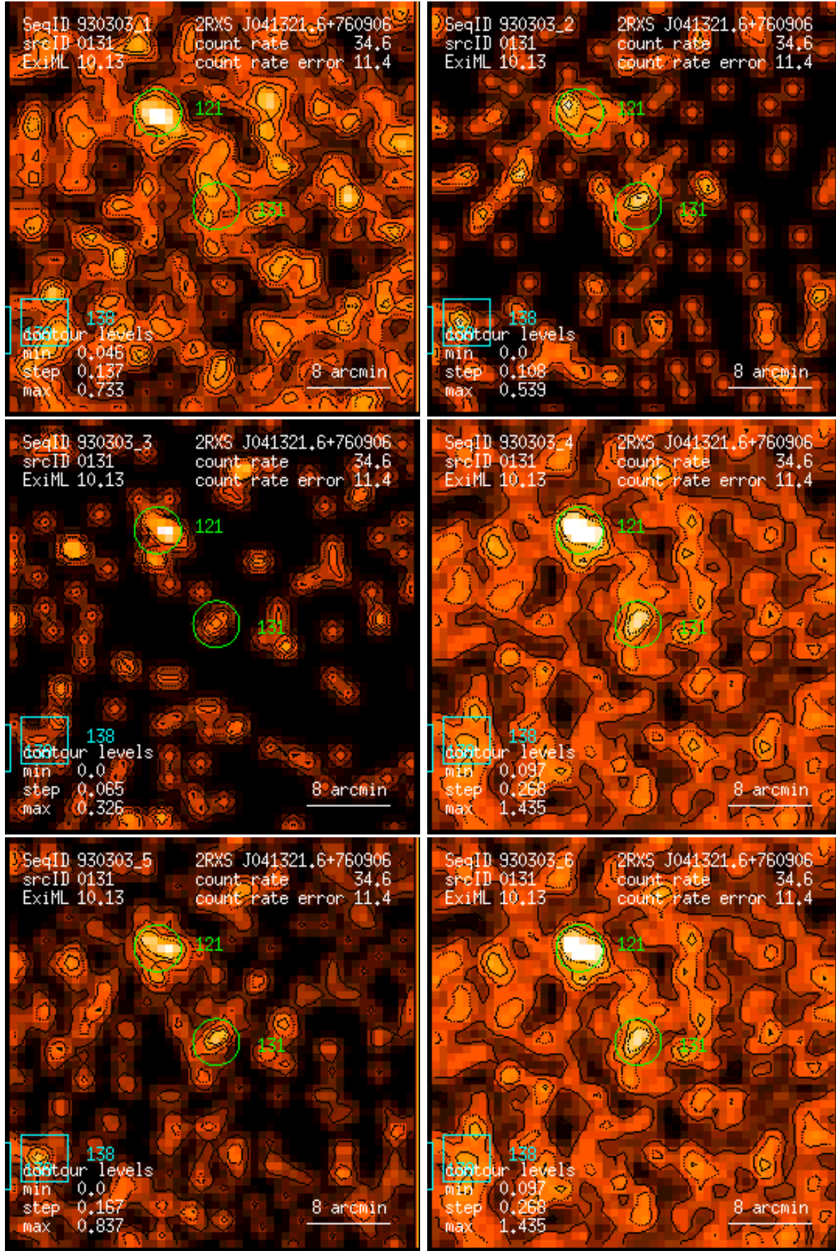
Figure 131: RASS 930303: detection 0131: band rate images, Gaussian filter: (1) PSPC channels 11 – 41, (2) 52 – 90, (3) 91 – 201, (4) 11 – 235, (5) 52 – 201, (6) 11 – 201. Broad band rates in counts/ks. Band rate contour levels in counts/ks/arcmin 2 .
