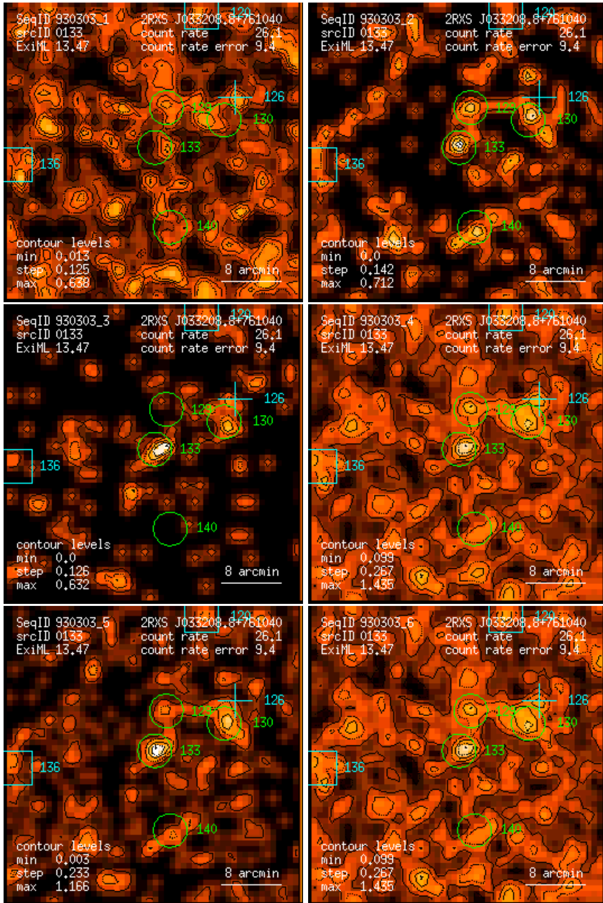
Figure 133: RASS 930303: detection 0133: band rate images, Gaussian filter: (1) PSPC channels 11 – 41, (2) 52 – 90, (3) 91 – 201, (4) 11 – 235, (5) 52 – 201, (6) 11 – 201. Broad band rates in counts/ks. Band rate contour levels in counts/ks/arcmin 2 .
