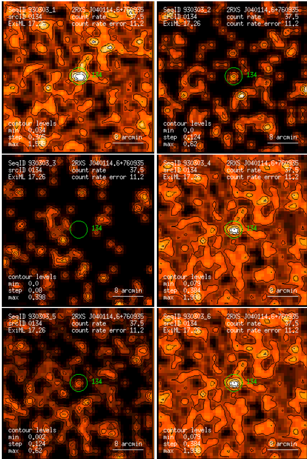
Figure 134: RASS 930303: detection 0134: band rate images, Gaussian filter: (1) PSPC channels 11 – 41, (2) 52 – 90, (3) 91 – 201, (4) 11 – 235, (5) 52 – 201, (6) 11 – 201. Broad band rates in counts/ks. Band rate contour levels in counts/ks/arcmin 2 .
