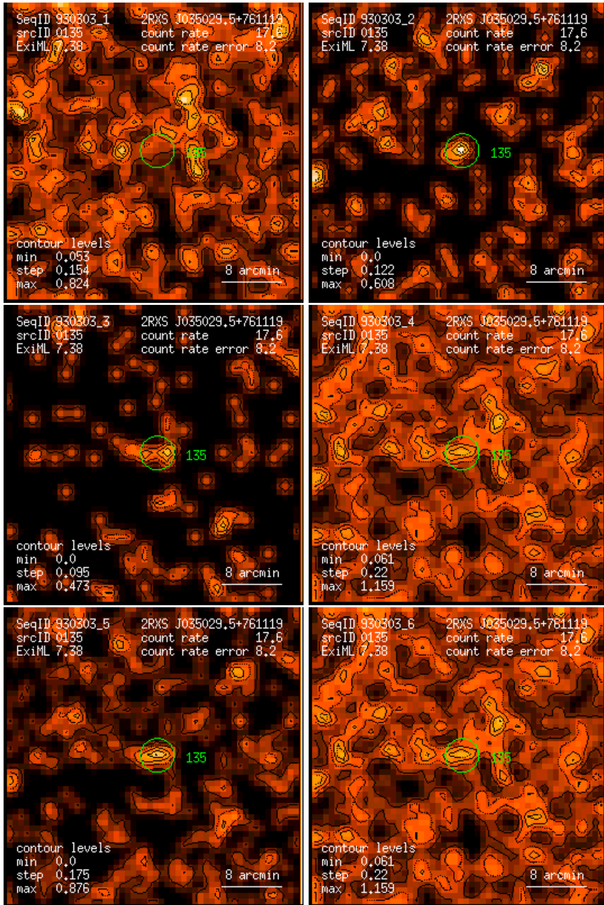
Figure 135: RASS 930303: detection 0135: band rate images, Gaussian filter: (1) PSPC channels 11 – 41, (2) 52 – 90, (3) 91 – 201, (4) 11 – 235, (5) 52 – 201, (6) 11 – 201. Broad band rates in counts/ks. Band rate contour levels in counts/ks/arcmin 2 .
