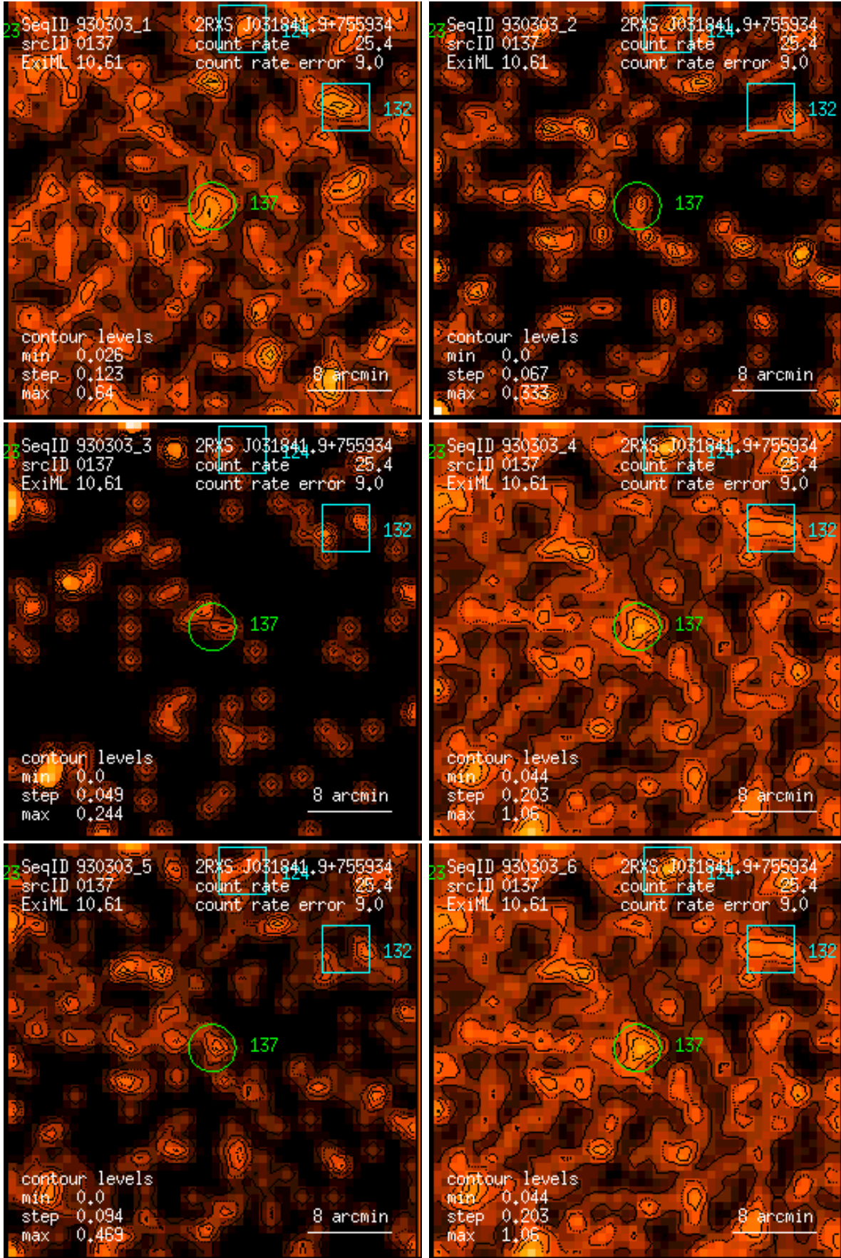
Figure 137: RASS 930303: detection 0137: band rate images, Gaussian filter: (1) PSPC channels 11 – 41, (2) 52 – 90, (3) 91 – 201, (4) 11 – 235, (5) 52 – 201, (6) 11 – 201. Broad band rates in counts/ks. Band rate contour levels in counts/ks/arcmin 2 .
