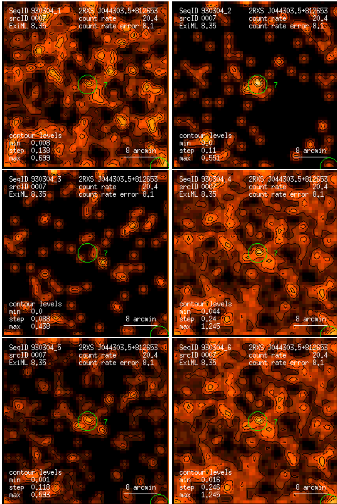
Figure 7: RASS 930304: detection 0007: band rate images, Gaussian filter: (1) PSPC channels 11 – 41, (2) 52 – 90, (3) 91 – 201, (4) 11 – 235, (5) 52 – 201, (6) 11 – 201. Broad band rates in counts/ks. Band rate contour levels in counts/ks/arcmin 2 .
