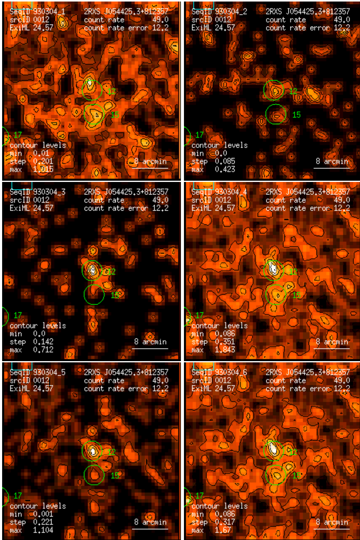
Figure 12: RASS 930304: detection 0012: band rate images, Gaussian filter: (1) PSPC channels 11 – 41, (2) 52 – 90, (3) 91 – 201, (4) 11 – 235, (5) 52 – 201, (6) 11 – 201. Broad band rates in counts/ks. Band rate contour levels in counts/ks/arcmin 2 .
