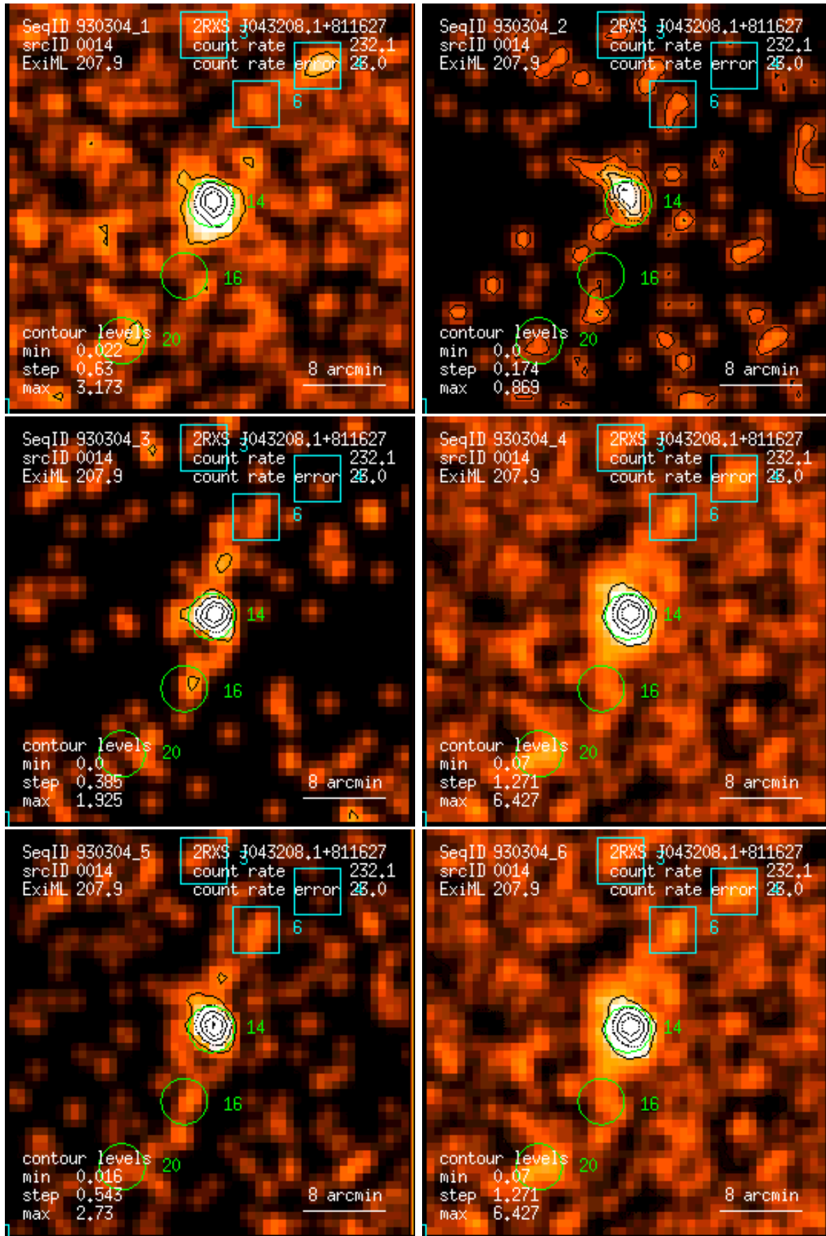
Figure 14: RASS 930304: detection 0014: band rate images, Gaussian filter: (1) PSPC channels 11 – 41, (2) 52 – 90, (3) 91 – 201, (4) 11 – 235, (5) 52 – 201, (6) 11 – 201. Broad band rates in counts/ks. Band rate contour levels in counts/ks/arcmin 2 .
