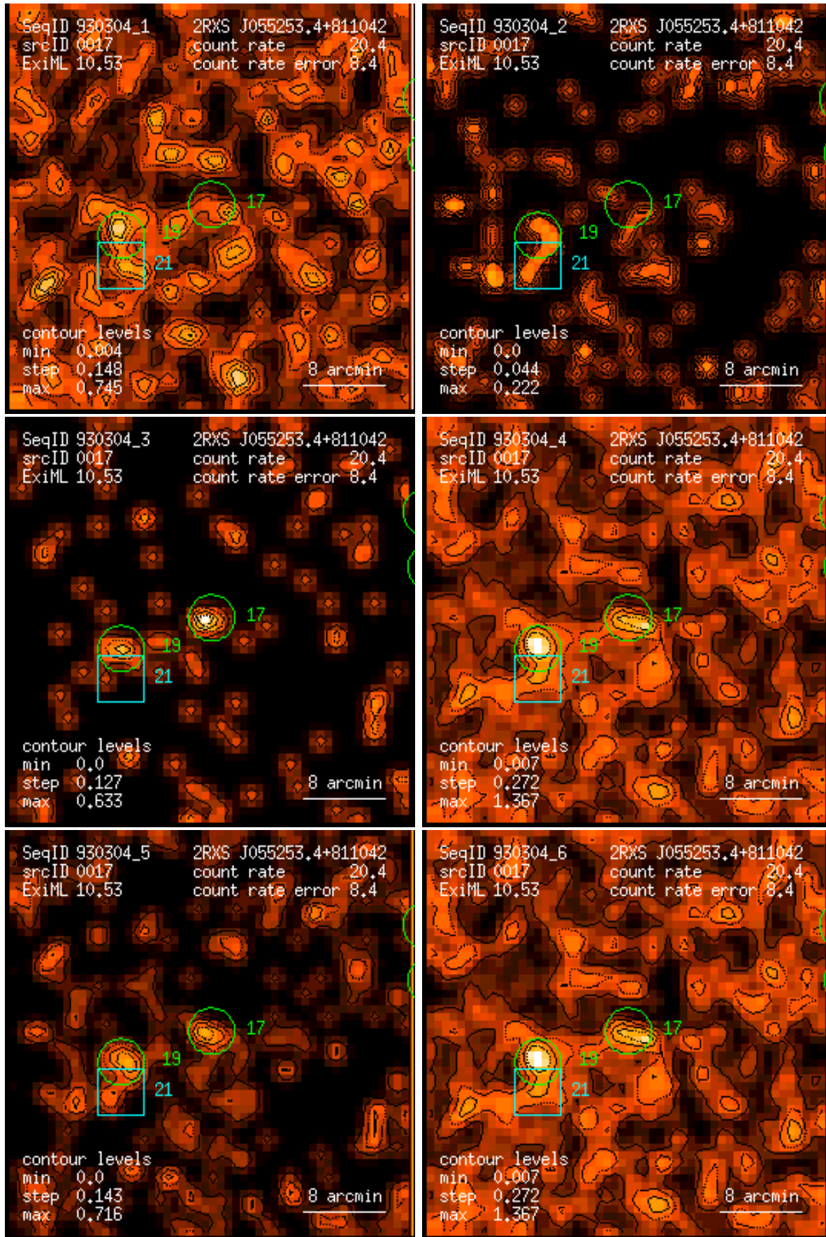
Figure 17: RASS 930304: detection 0017: band rate images, Gaussian filter: (1) PSPC channels 11 – 41, (2) 52 – 90, (3) 91 – 201, (4) 11 – 235, (5) 52 – 201, (6) 11 – 201. Broad band rates in counts/ks. Band rate contour levels in counts/ks/arcmin 2 .
