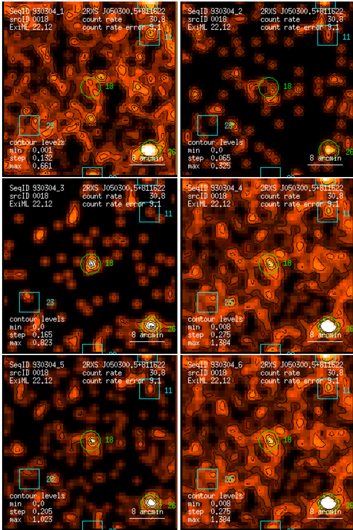
Figure 18: RASS 930304: detection 0018: band rate images, Gaussian filter: (1) PSPC channels 11 – 41, (2) 52 – 90, (3) 91 – 201, (4) 11 – 235, (5) 52 – 201, (6) 11 – 201. Broad band rates in counts/ks. Band rate contour levels in counts/ks/arcmin 2 .
