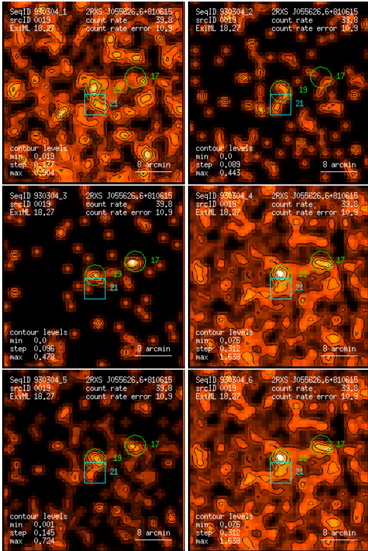
Figure 19: RASS 930304: detection 0019: band rate images, Gaussian filter: (1) PSPC channels 11 – 41, (2) 52 – 90, (3) 91 – 201, (4) 11 – 235, (5) 52 – 201, (6) 11 – 201. Broad band rates in counts/ks. Band rate contour levels in counts/ks/arcmin 2 .
