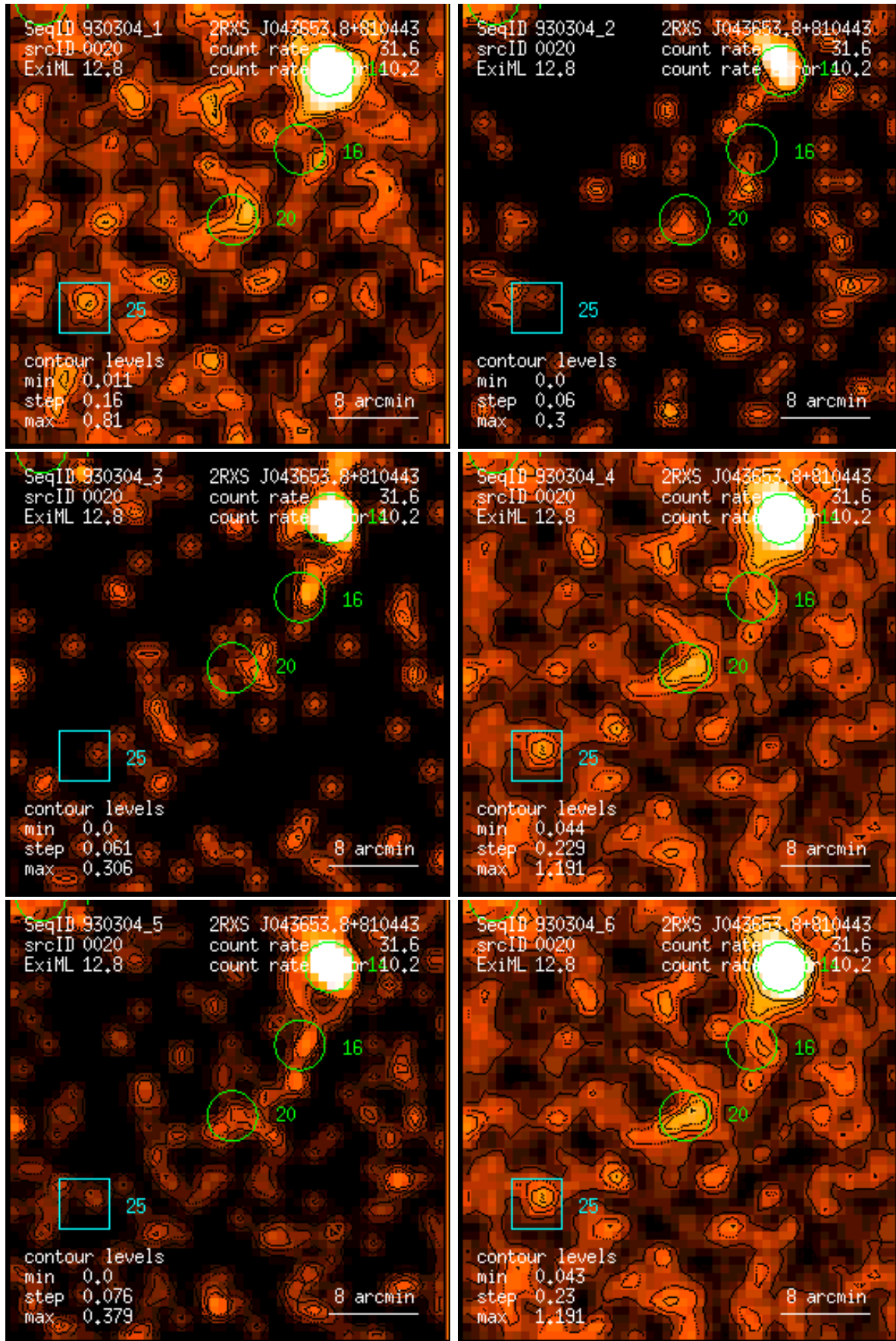
Figure 20: RASS 930304: detection 0020: band rate images, Gaussian filter: (1) PSPC channels 11 – 41, (2) 52 – 90, (3) 91 – 201, (4) 11 – 235, (5) 52 – 201, (6) 11 – 201. Broad band rates in counts/ks. Band rate contour levels in counts/ks/arcmin 2 .
