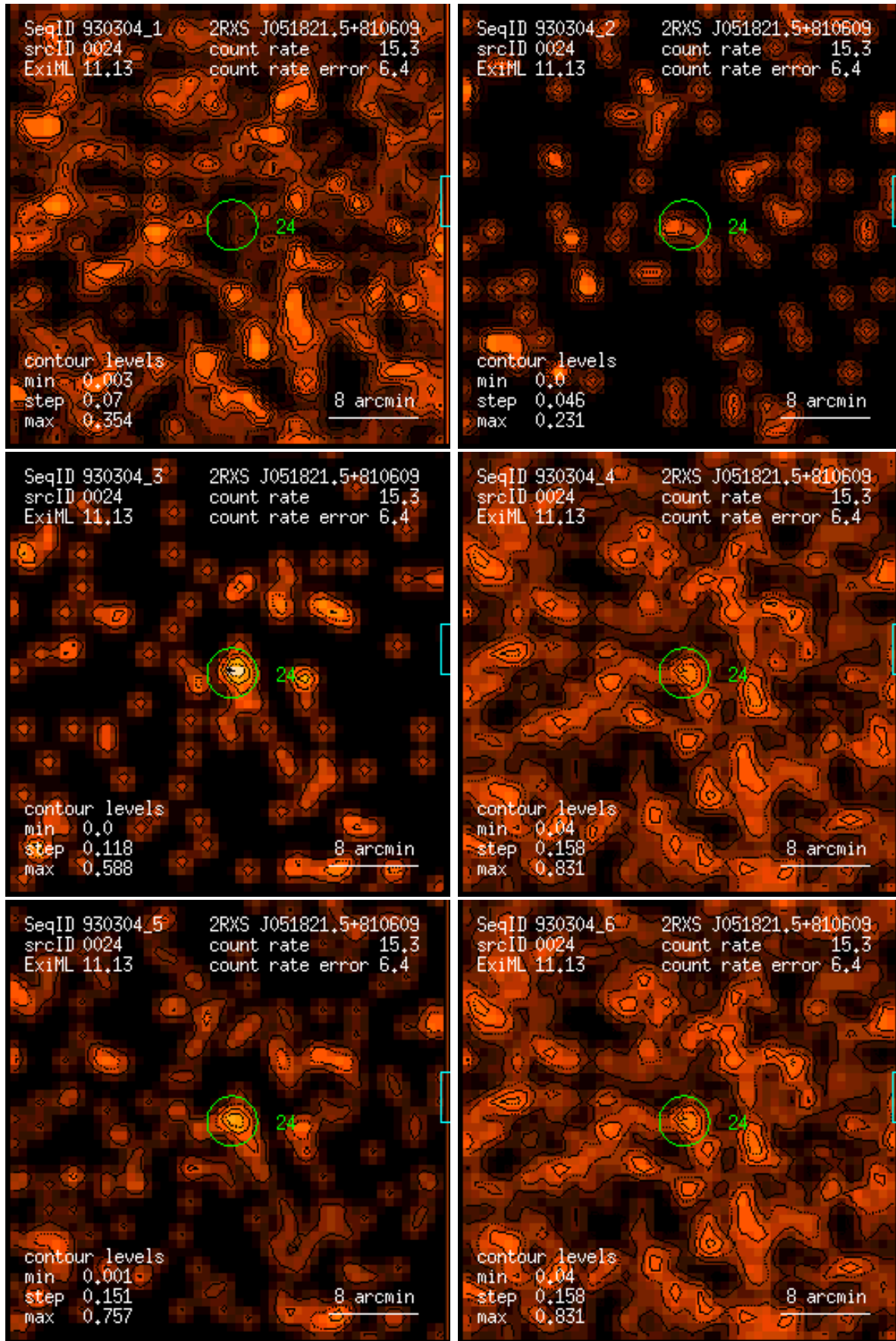
Figure 24: RASS 930304: detection 0024: band rate images, Gaussian filter: (1) PSPC channels 11 – 41, (2) 52 – 90, (3) 91 – 201, (4) 11 – 235, (5) 52 – 201, (6) 11 – 201. Broad band rates in counts/ks. Band rate contour levels in counts/ks/arcmin 2 .
