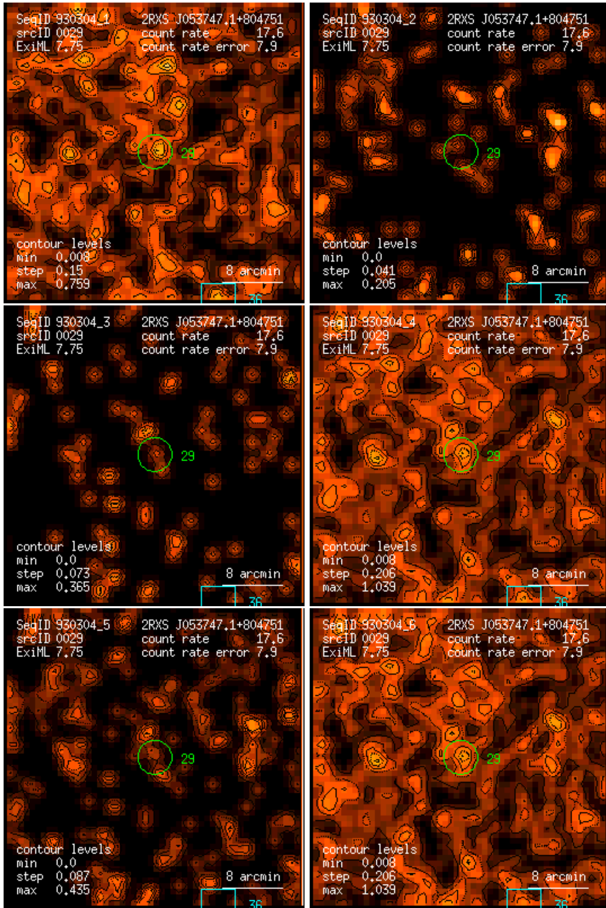
Figure 29: RASS 930304: detection 0029: band rate images, Gaussian filter: (1) PSPC channels 11 – 41, (2) 52 – 90, (3) 91 – 201, (4) 11 – 235, (5) 52 – 201, (6) 11 – 201. Broad band rates in counts/ks. Band rate contour levels in counts/ks/arcmin 2 .
