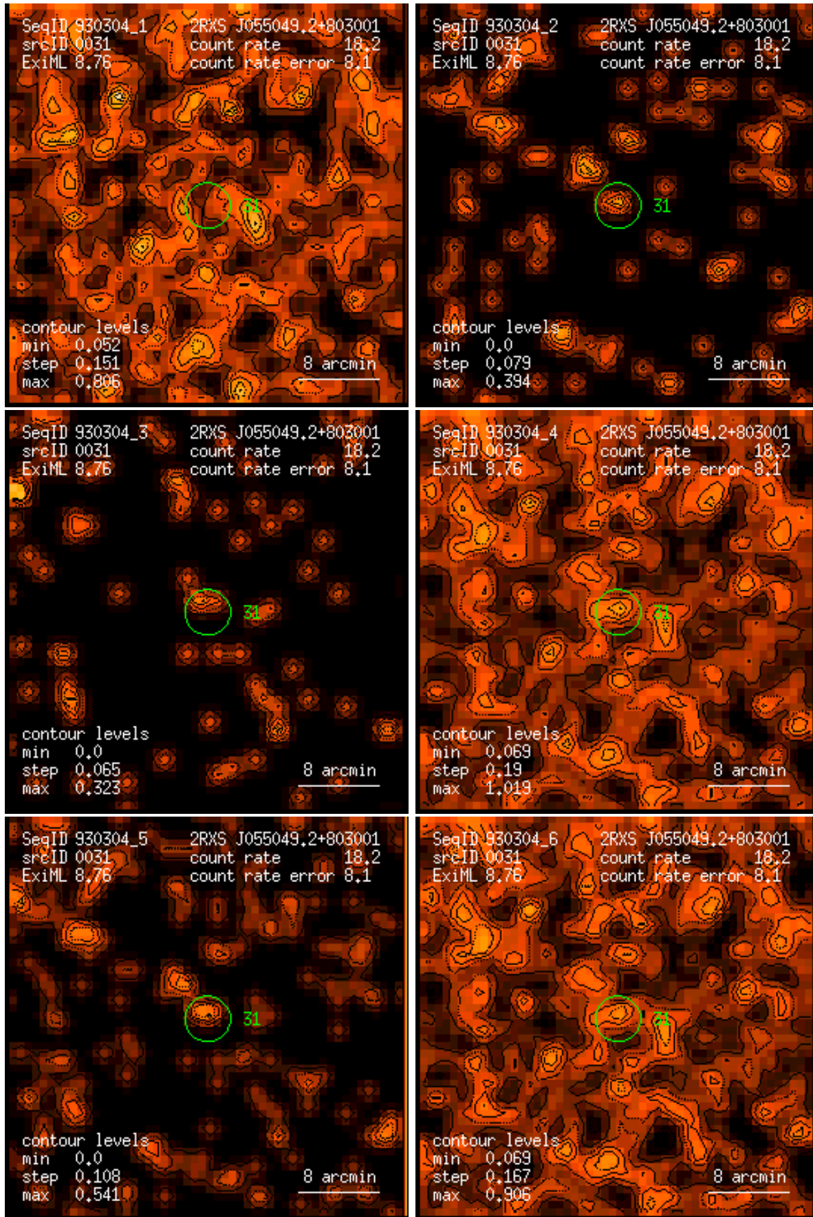
Figure 31: RASS 930304: detection 0031: band rate images, Gaussian filter: (1) PSPC channels 11 – 41, (2) 52 – 90, (3) 91 – 201, (4) 11 – 235, (5) 52 – 201, (6) 11 – 201. Broad band rates in counts/ks. Band rate contour levels in counts/ks/arcmin 2 .
