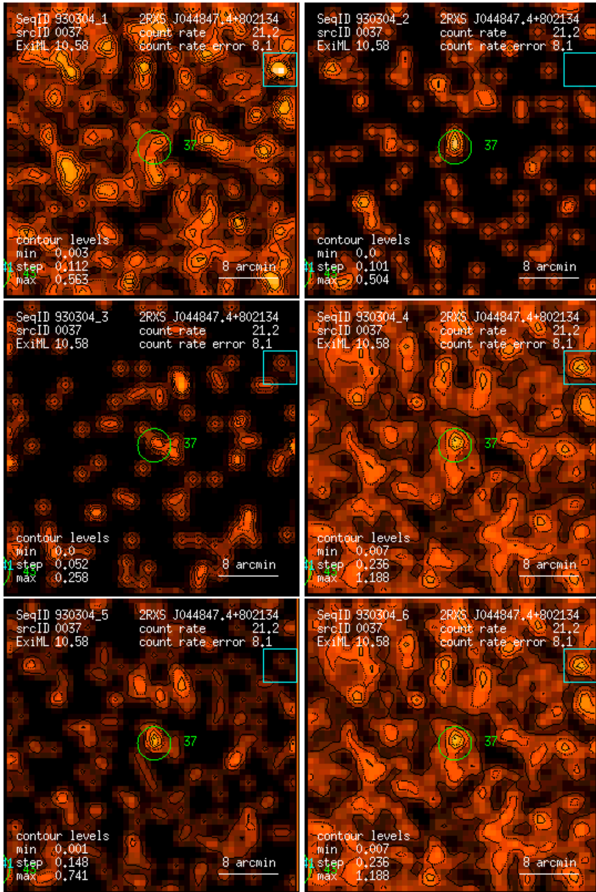
Figure 37: RASS 930304: detection 0037: band rate images, Gaussian filter: (1) PSPC channels 11 – 41, (2) 52 – 90, (3) 91 – 201, (4) 11 – 235, (5) 52 – 201, (6) 11 – 201. Broad band rates in counts/ks. Band rate contour levels in counts/ks/arcmin 2 .
