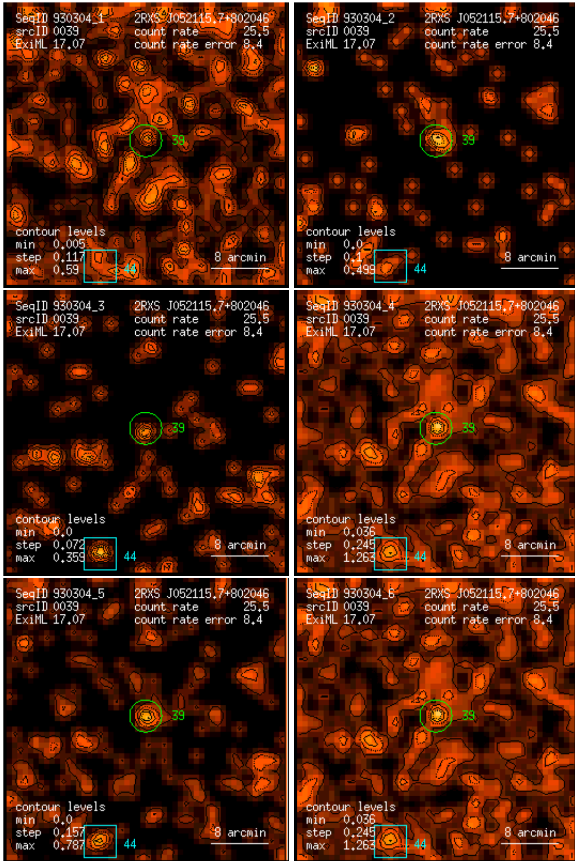
Figure 39: RASS 930304: detection 0039: band rate images, Gaussian filter: (1) PSPC channels 11 – 41, (2) 52 – 90, (3) 91 – 201, (4) 11 – 235, (5) 52 – 201, (6) 11 – 201. Broad band rates in counts/ks. Band rate contour levels in counts/ks/arcmin 2 .
