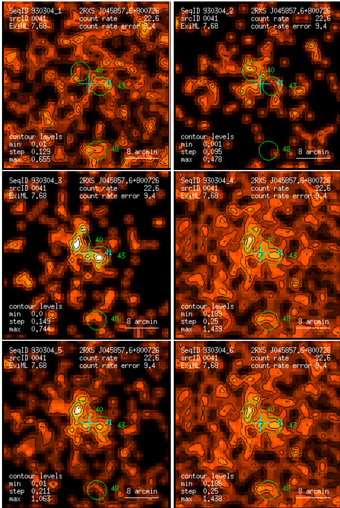
Figure 41: RASS 930304: detection 0041: band rate images, Gaussian filter: (1) PSPC channels 11 – 41, (2) 52 – 90, (3) 91 – 201, (4) 11 – 235, (5) 52 – 201, (6) 11 – 201. Broad band rates in counts/ks. Band rate contour levels in counts/ks/arcmin 2 .
