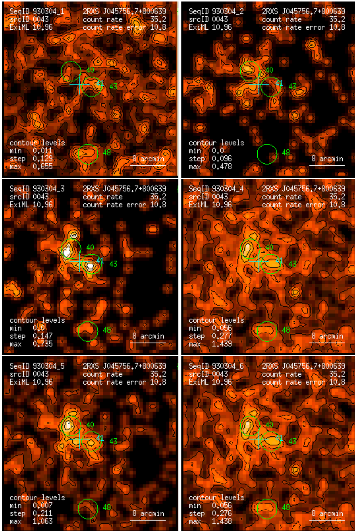
Figure 43: RASS 930304: detection 0043: band rate images, Gaussian filter: (1) PSPC channels 11 – 41, (2) 52 – 90, (3) 91 – 201, (4) 11 – 235, (5) 52 – 201, (6) 11 – 201. Broad band rates in counts/ks. Band rate contour levels in counts/ks/arcmin 2 .
