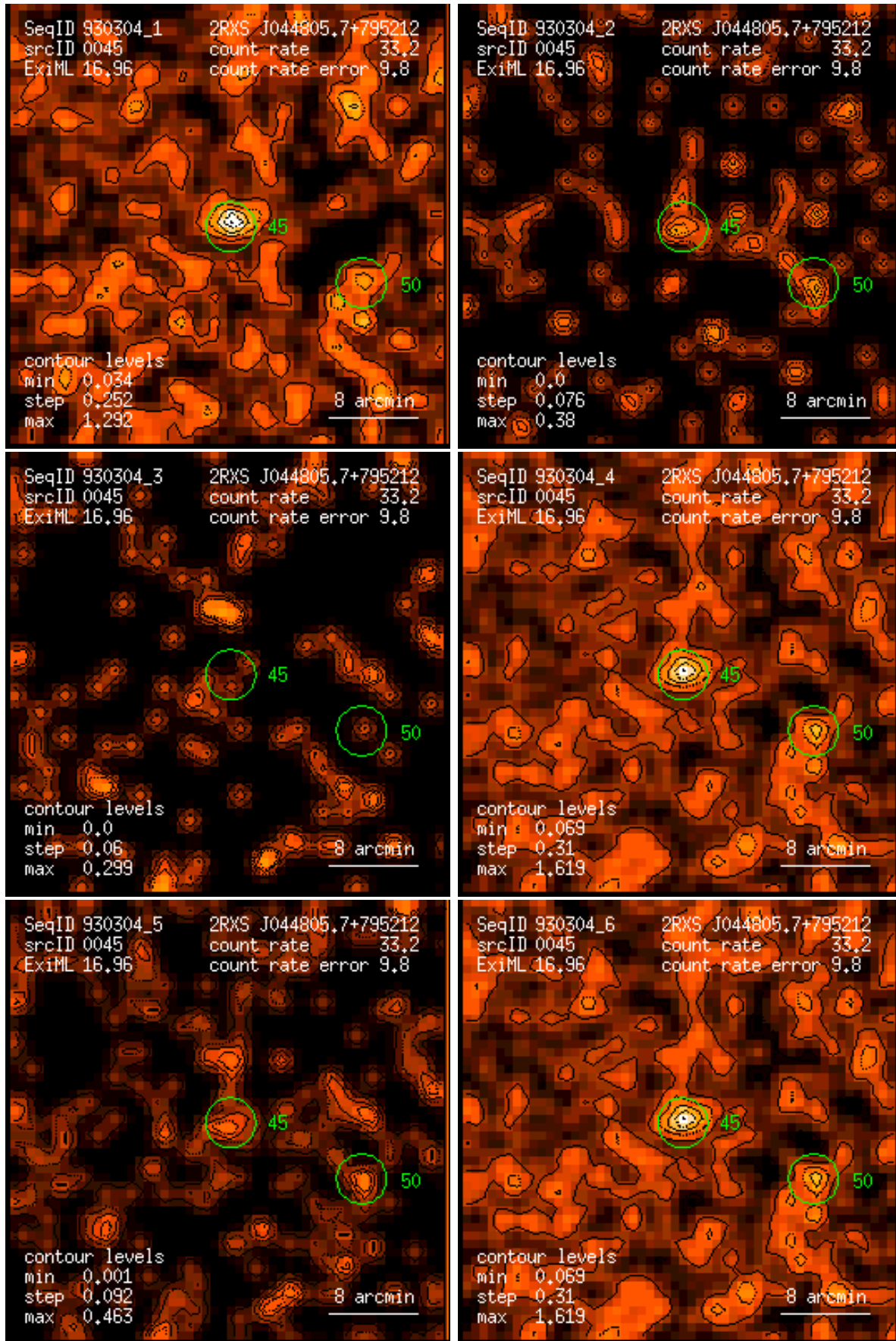
Figure 45: RASS 930304: detection 0045: band rate images, Gaussian filter: (1) PSPC channels 11 – 41, (2) 52 – 90, (3) 91 – 201, (4) 11 – 235, (5) 52 – 201, (6) 11 – 201. Broad band rates in counts/ks. Band rate contour levels in counts/ks/arcmin 2 .
