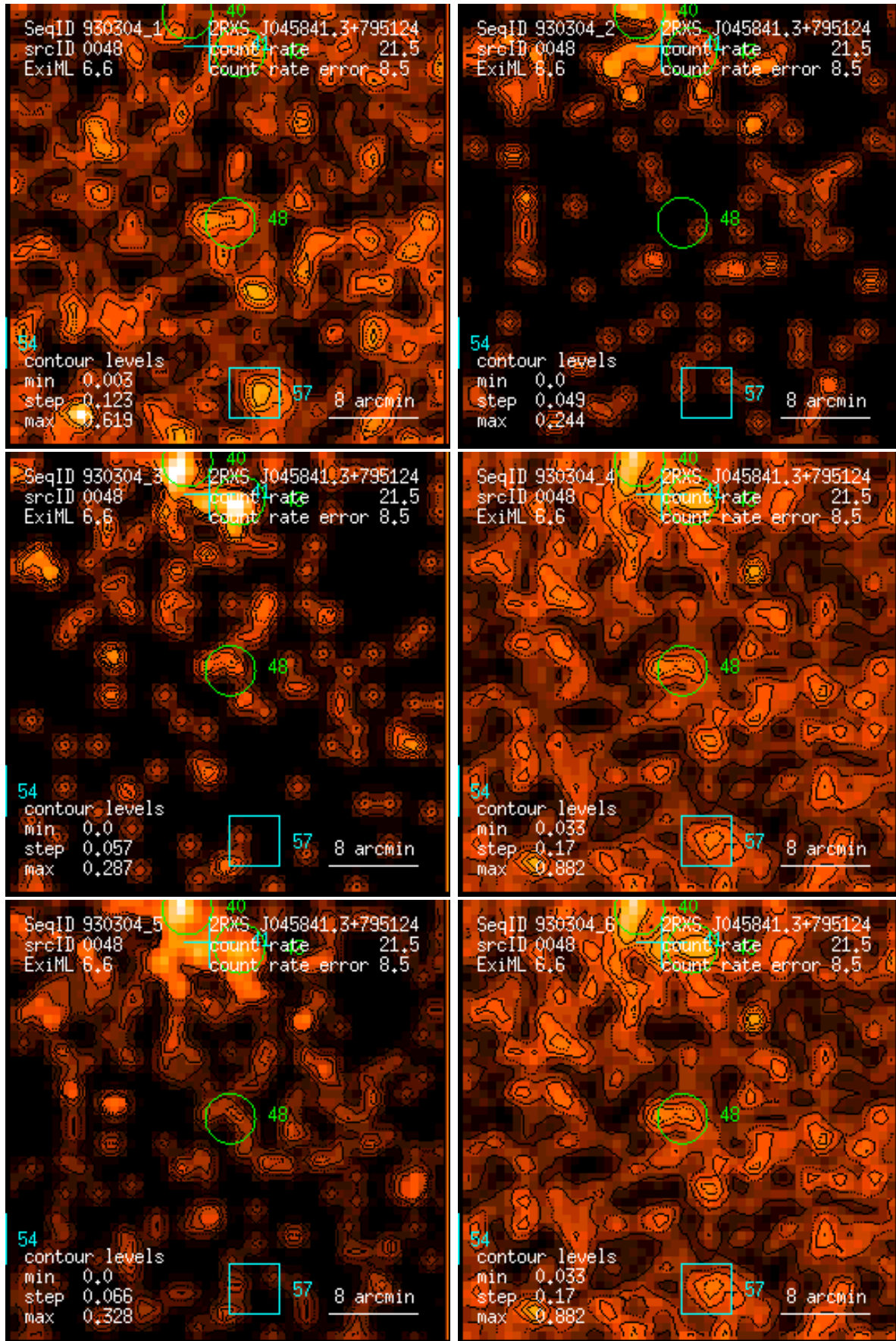
Figure 48: RASS 930304: detection 0048: band rate images, Gaussian filter: (1) PSPC channels 11 – 41, (2) 52 – 90, (3) 91 – 201, (4) 11 – 235, (5) 52 – 201, (6) 11 – 201. Broad band rates in counts/ks. Band rate contour levels in counts/ks/arcmin 2 .
