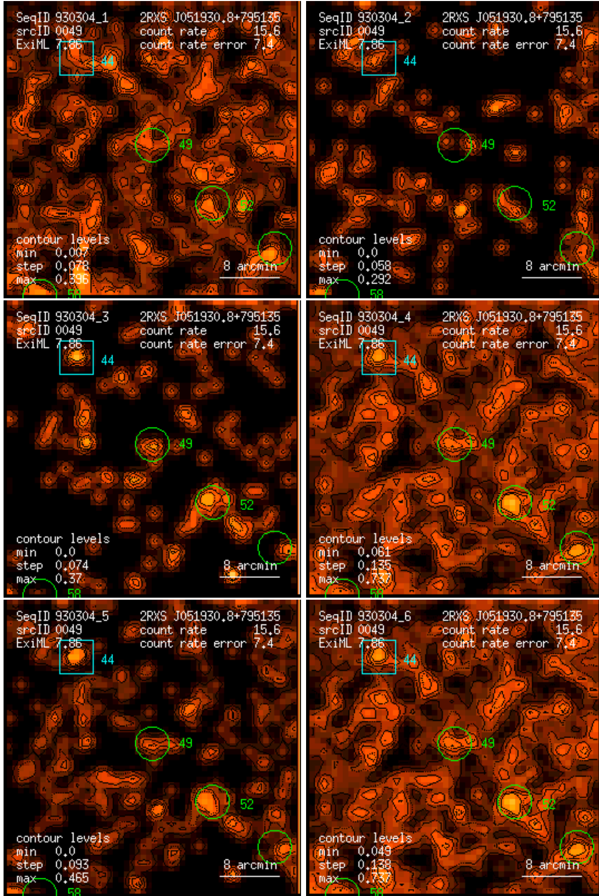
Figure 49: RASS 930304: detection 0049: band rate images, Gaussian filter: (1) PSPC channels 11 – 41, (2) 52 – 90, (3) 91 – 201, (4) 11 – 235, (5) 52 – 201, (6) 11 – 201. Broad band rates in counts/ks. Band rate contour levels in counts/ks/arcmin 2 .
