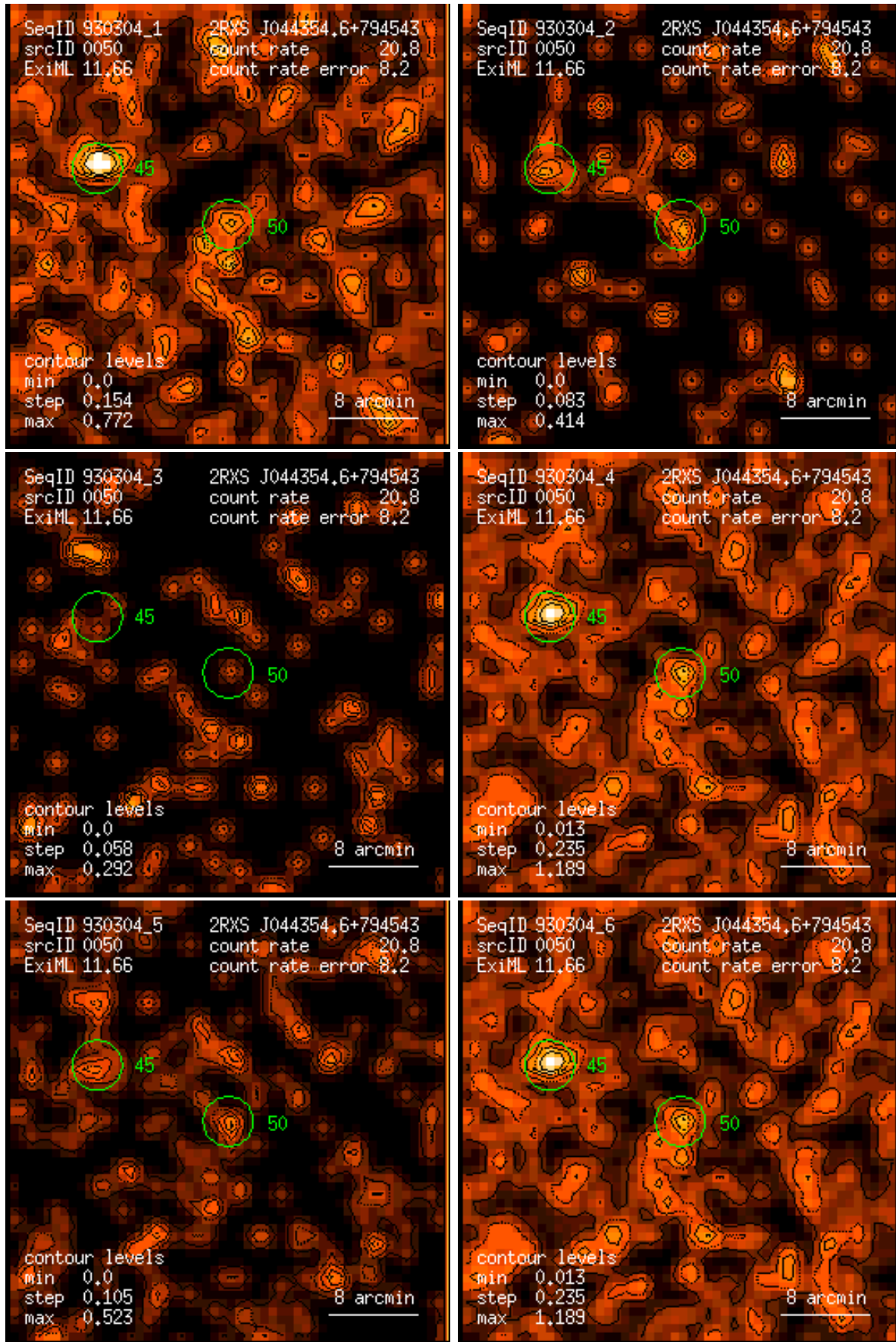
Figure 50: RASS 930304: detection 0050: band rate images, Gaussian filter: (1) PSPC channels 11 – 41, (2) 52 – 90, (3) 91 – 201, (4) 11 – 235, (5) 52 – 201, (6) 11 – 201. Broad band rates in counts/ks. Band rate contour levels in counts/ks/arcmin 2 .
