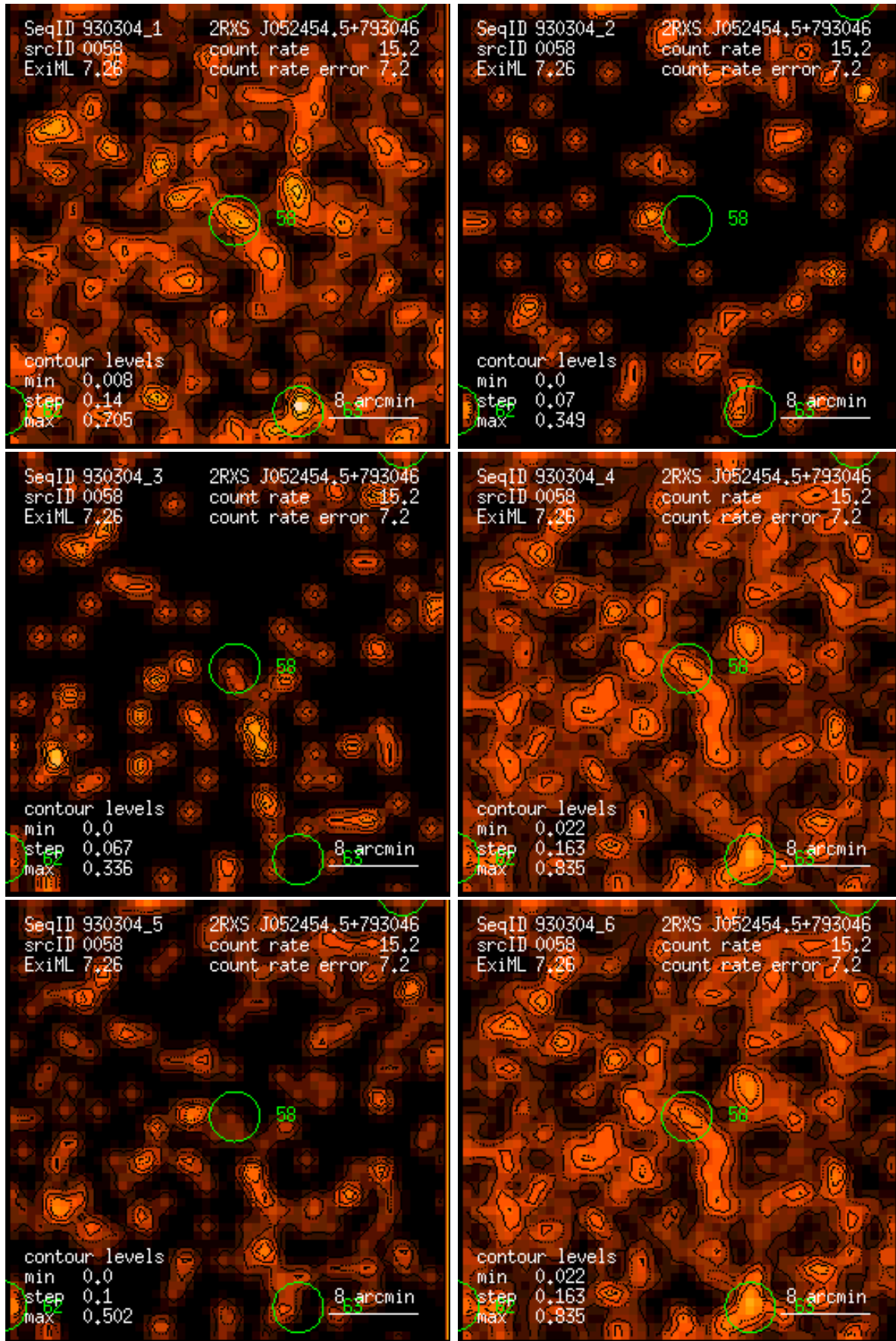
Figure 58: RASS 930304: detection 0058: band rate images, Gaussian filter: (1) PSPC channels 11 – 41, (2) 52 – 90, (3) 91 – 201, (4) 11 – 235, (5) 52 – 201, (6) 11 – 201. Broad band rates in counts/ks. Band rate contour levels in counts/ks/arcmin 2 .
