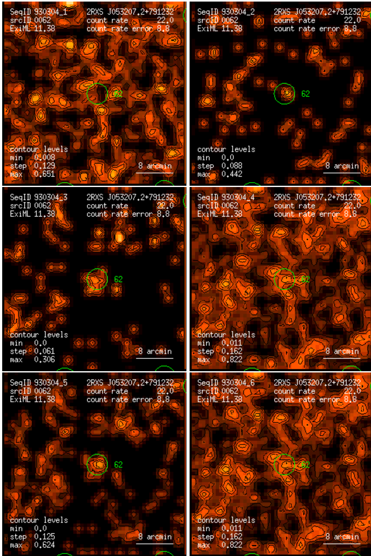
Figure 62: RASS 930304: detection 0062: band rate images, Gaussian filter: (1) PSPC channels 11 – 41, (2) 52 – 90, (3) 91 – 201, (4) 11 – 235, (5) 52 – 201, (6) 11 – 201. Broad band rates in counts/ks. Band rate contour levels in counts/ks/arcmin 2 .
