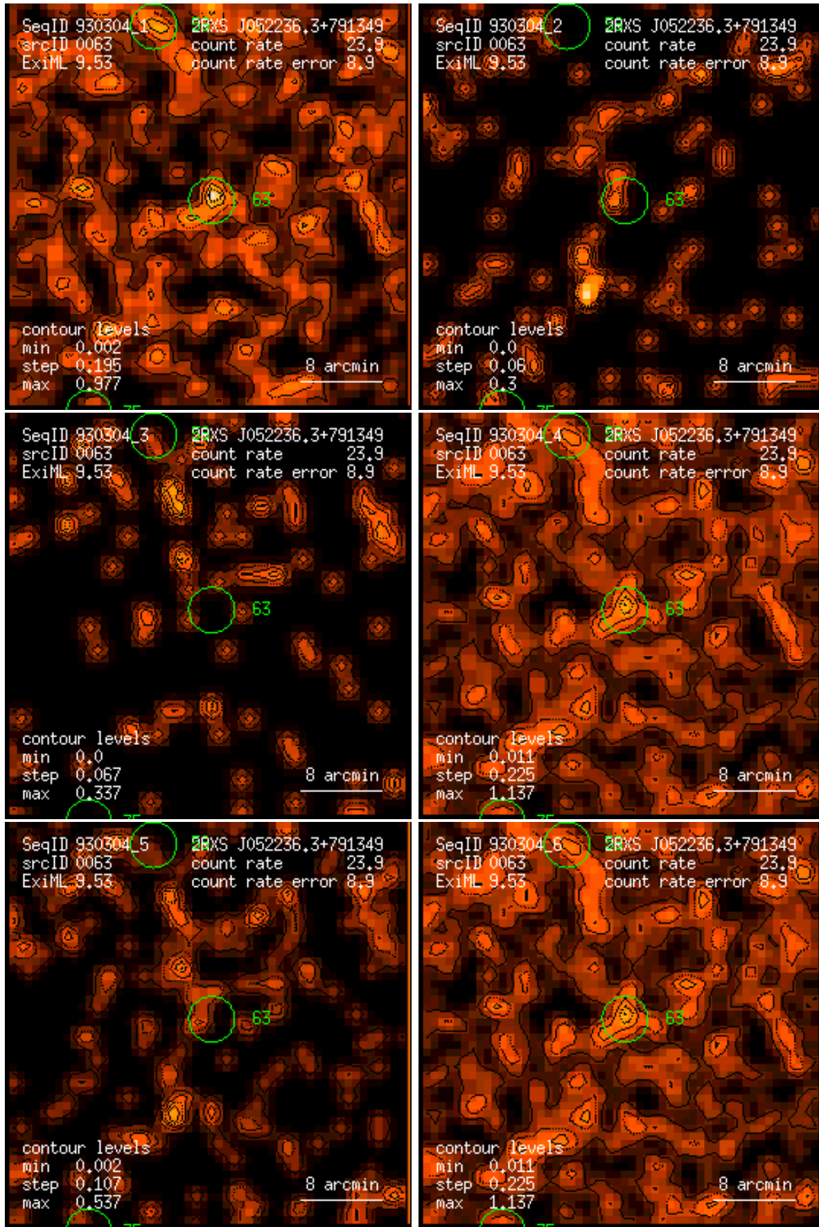
Figure 63: RASS 930304: detection 0063: band rate images, Gaussian filter: (1) PSPC channels 11 – 41, (2) 52 – 90, (3) 91 – 201, (4) 11 – 235, (5) 52 – 201, (6) 11 – 201. Broad band rates in counts/ks. Band rate contour levels in counts/ks/arcmin 2 .
